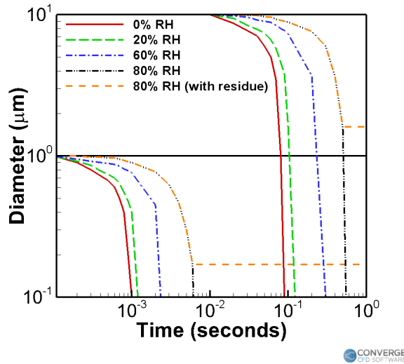
FIG. 1: Changes to water droplet diameter as a result of evaporation, taken for two different initial droplet sizes (1 and 10 \mu\text{m} ) and for different conditions of relative humidity (RH), as shown in the study of Morawksa 7 .
