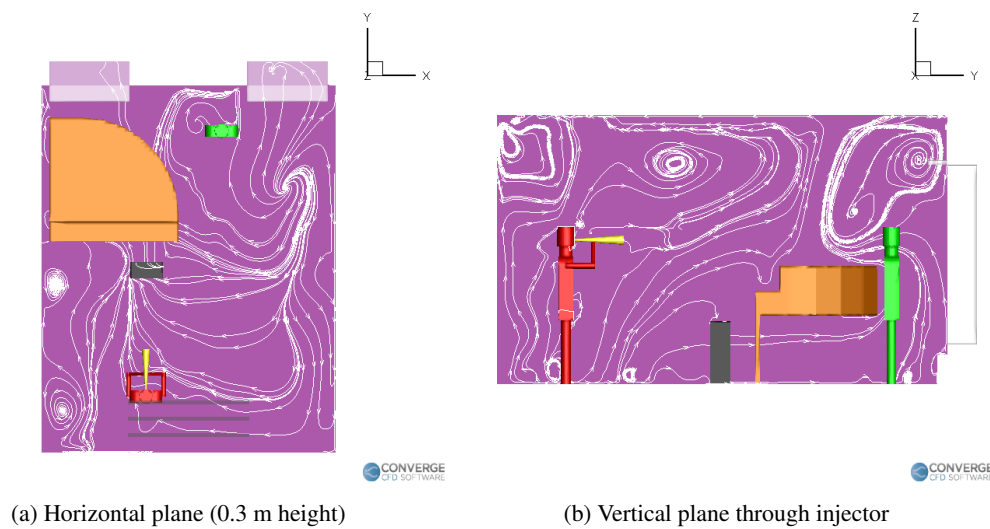
FIG. 14: Airflow streamlines inside the room with a purifier on the ground.
