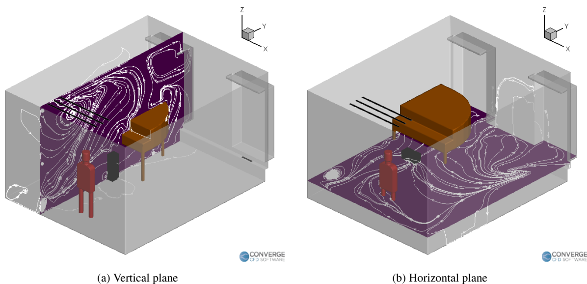
FIG. 5: Airflow streamlines inside the room with a singer and a purifier.
