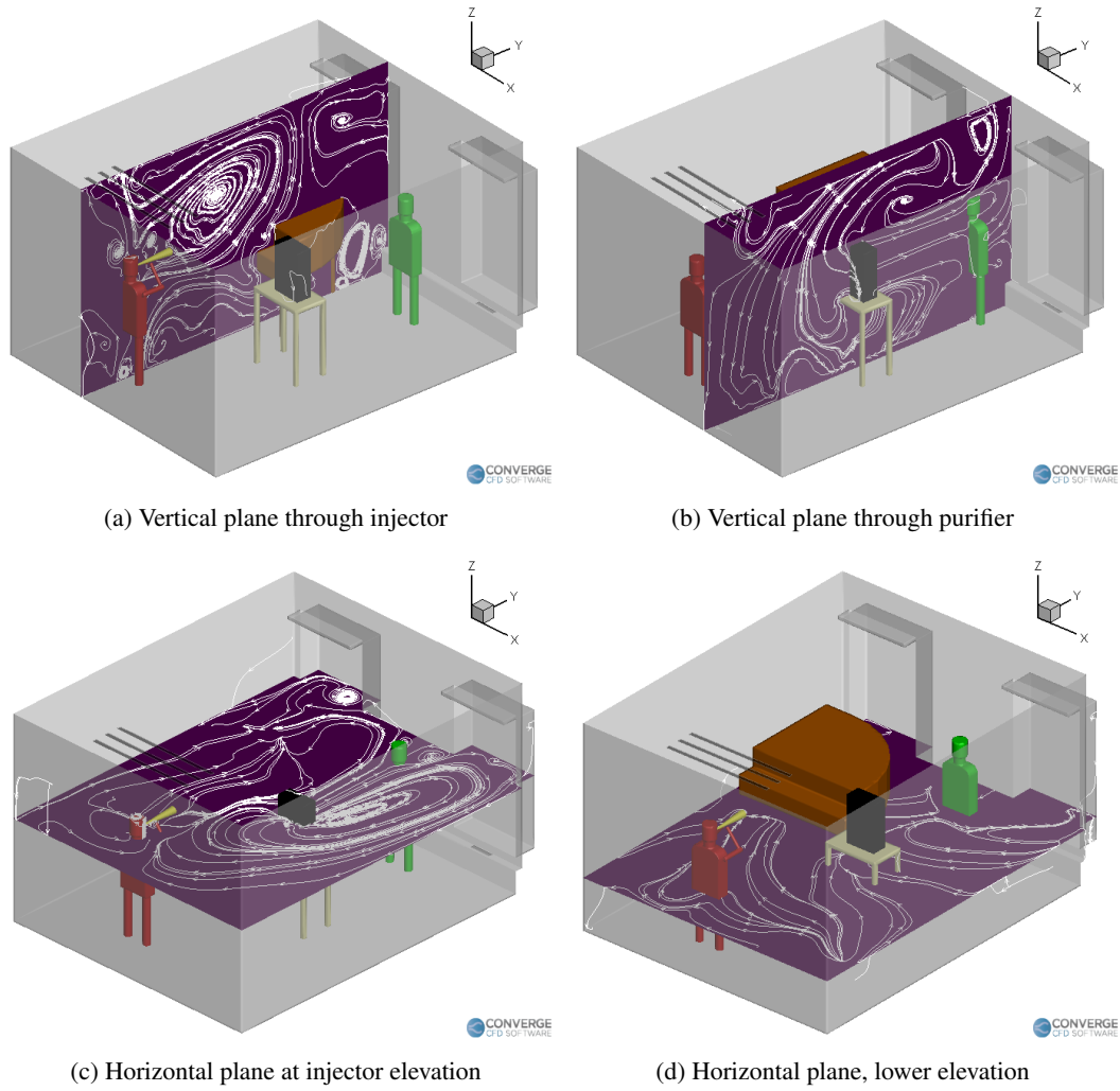
FIG. 13: Airflow streamlines inside the room with a purifier on the right table.
