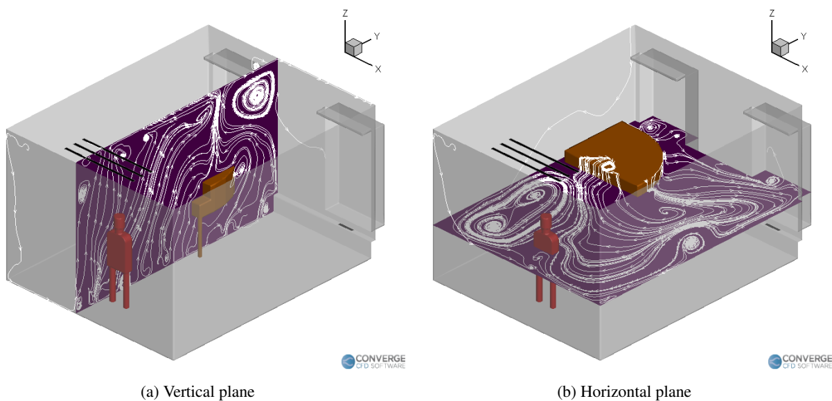
FIG. 4: Airflow streamlines inside the room with a singer but without a purifier.
