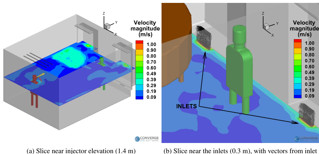
FIG. 11: Time averaged velocity magnitude contours for the no purifier case.
