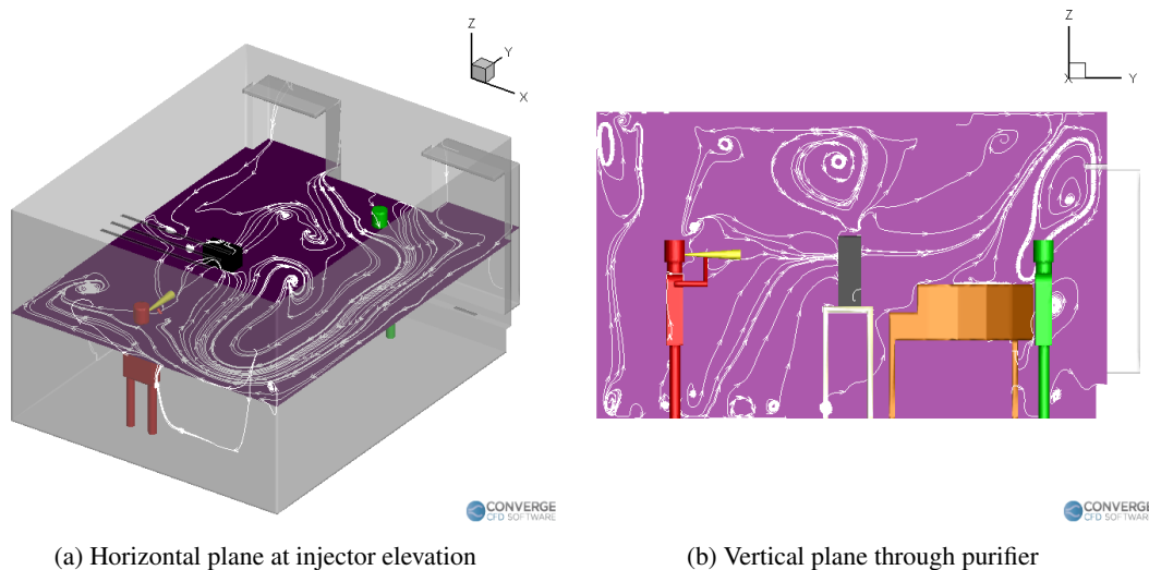
FIG. 12: Airflow streamlines inside the room with a purifier on the left table.
