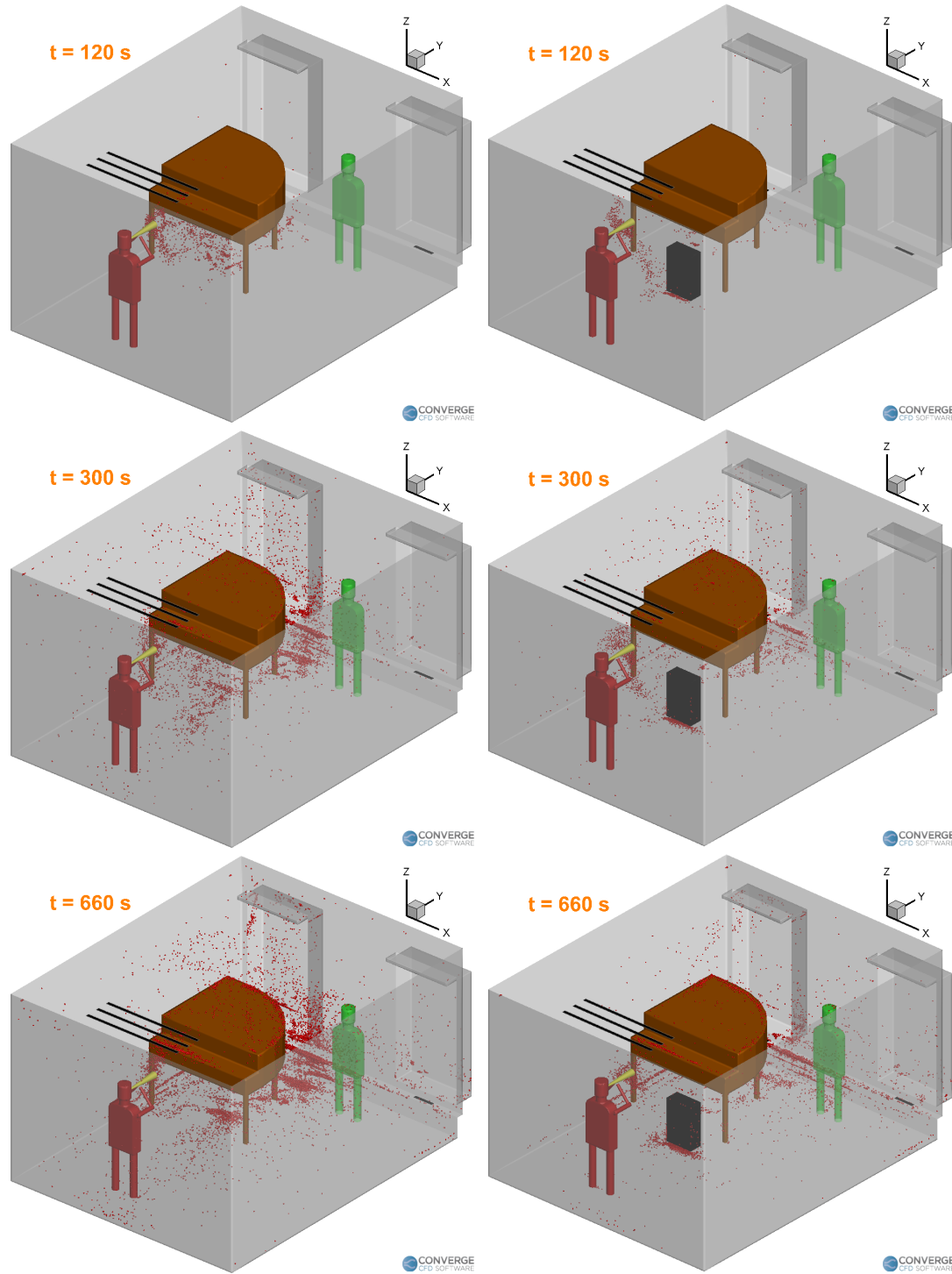
FIG. 8: Aerosol cloud profiles at three instances of time inside the room: left side without a purifier; right side with a purifier on the ground.
