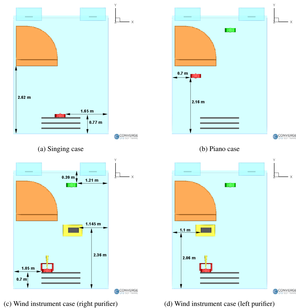
FIG. 3: Locations of the student, teacher and purifier in the different scenarios.
