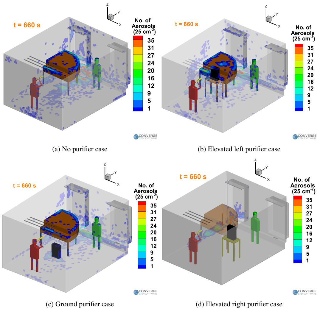
FIG. 9: Deposition trends for the wind instrument (trombone) case.
