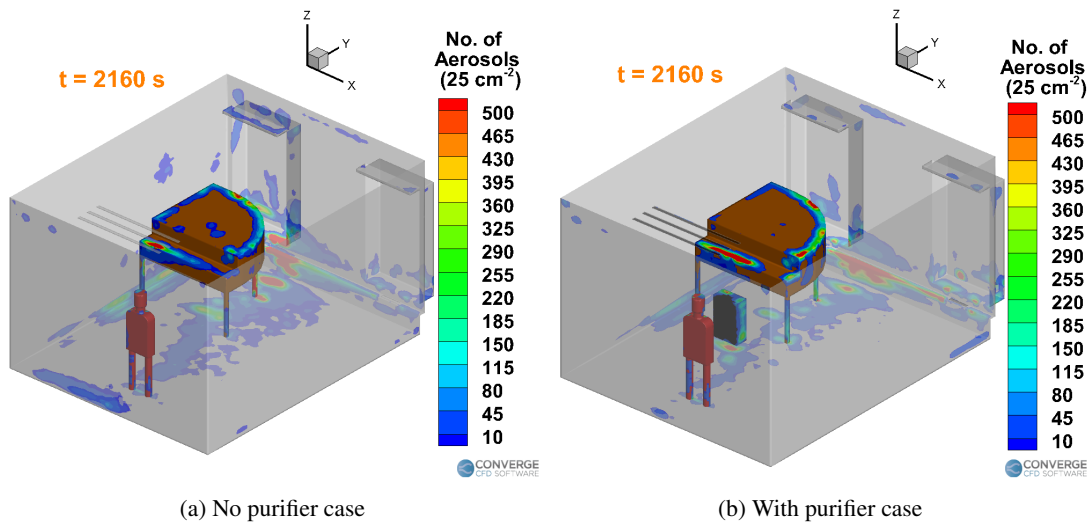
FIG. 6: Aerosol deposition per unit cell area ( 25 \text{ cm}^2 ) inside the room with a singer.
