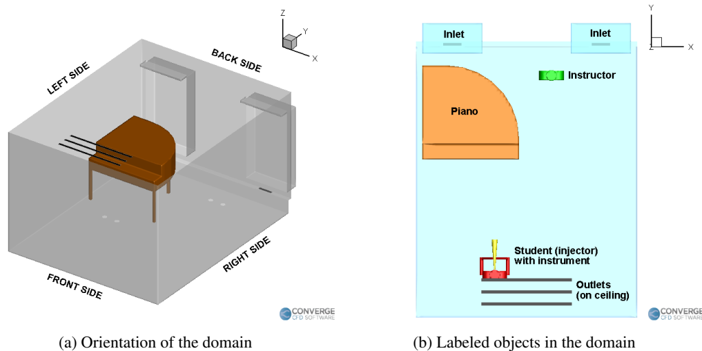
FIG. 2: Orientation and objects in the domain.
