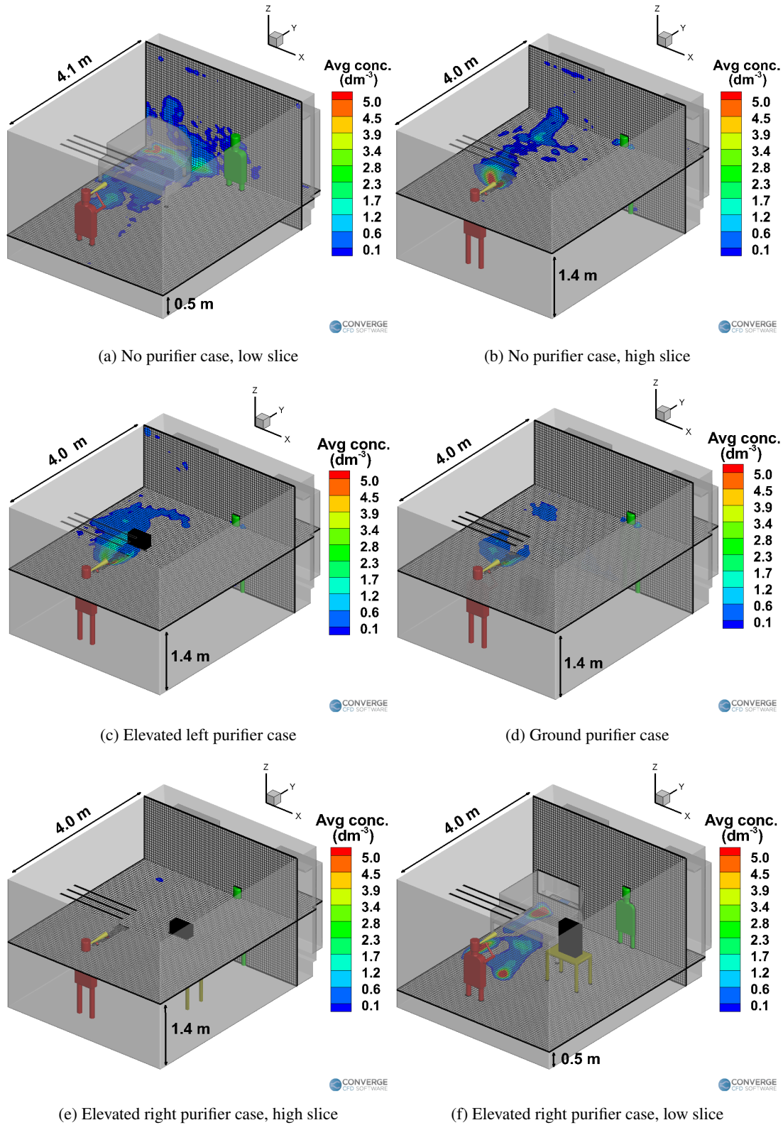
FIG. 16: Time averaged airborne aerosol concentrations (per cubic decimeter) for the wind instrument (trombone) cases.
