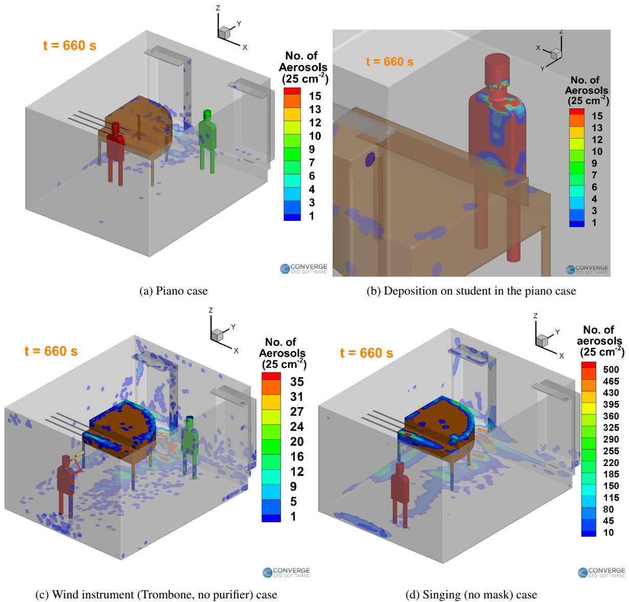
FIG. 18: Comparison of the deposition of aerosols inside the domain between the three types of musical sessions.
