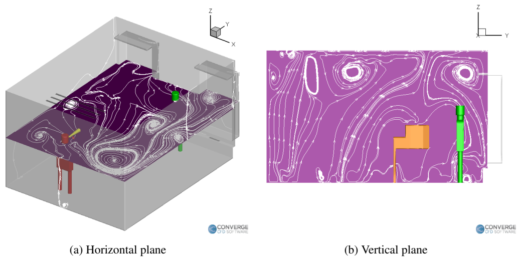
FIG. 10: Airflow streamlines inside the room (no purifier case).
