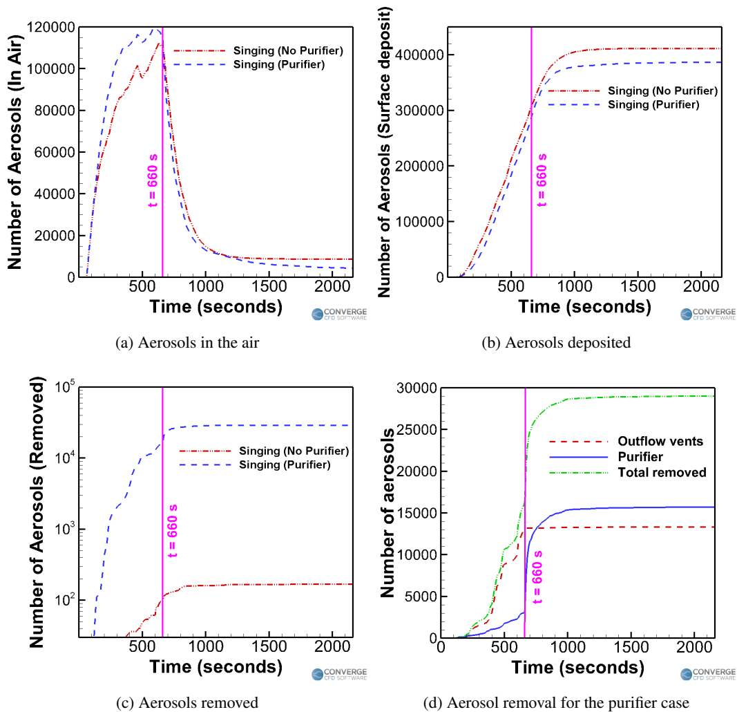
FIG. 7: Trend comparison for the singing cases.
