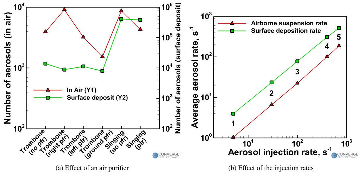
FIG. 19: Summarizing the observed trends.
