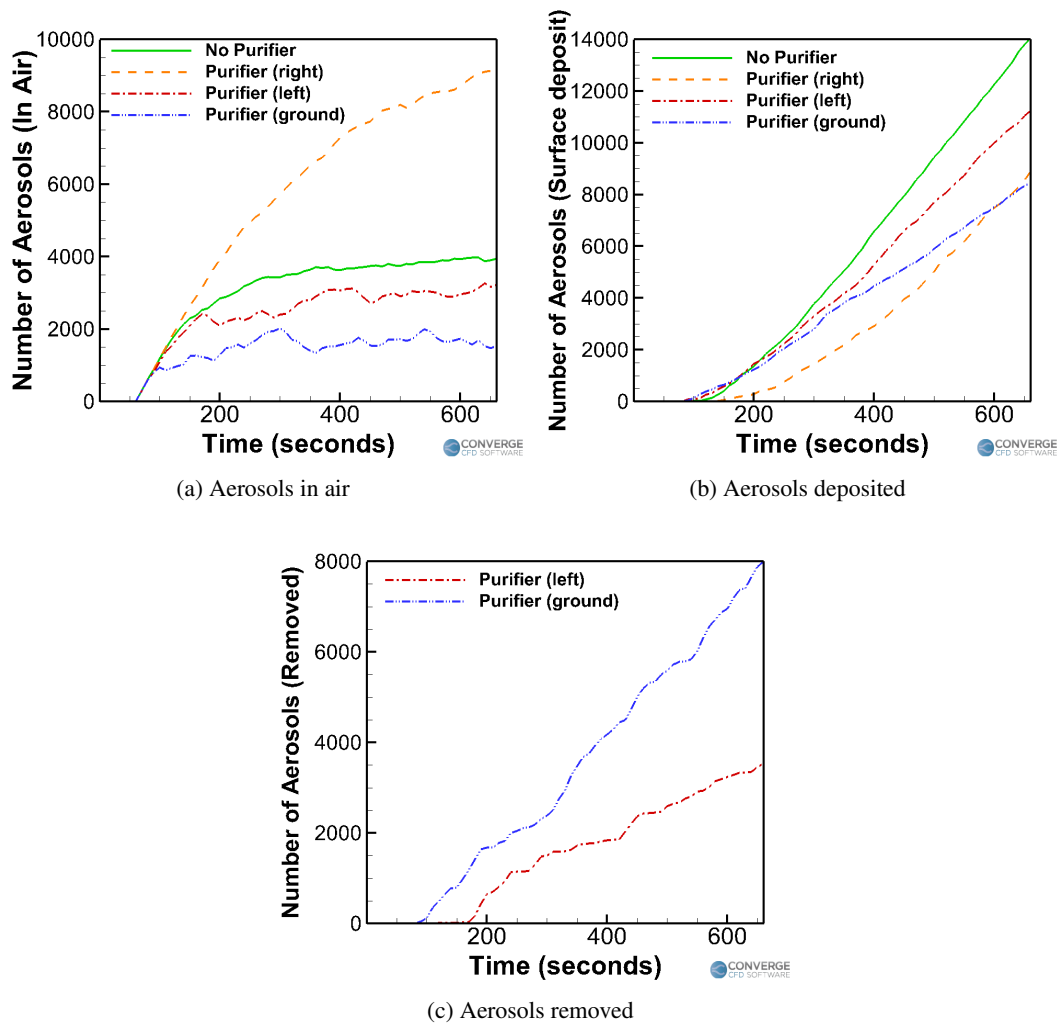
FIG. 15: Trend comparison for the wind instrument (trombone) cases.
