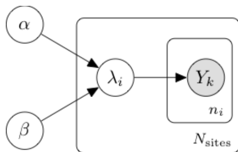
Figure 1. Graphical representation of the adverse event reporting model
