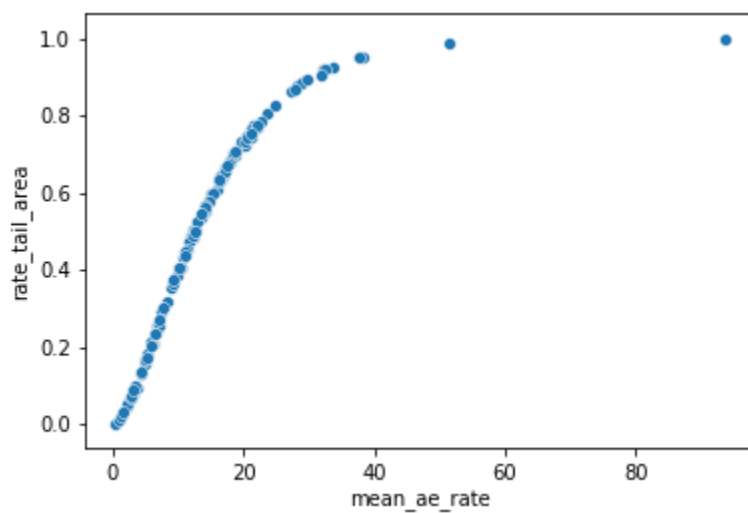
Fig. 2 - The rate tail area risk metric as a function of the posterior mean site rate.
