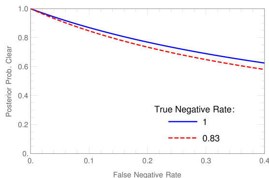
Figure 4: In an extremely high prevalence of 0.6 (60k cases per 100k population) such as in a hospital, jail, or some other sealed outbreak cluster, these curves show that a false negative rate of < 0.05 is needed for a useful test to rule out infection with 95% confidence, i.e. a sensitivity of > 95\% . This result is not strongly affected by the specificity, as shown by the two curves indicating a perfect test (specificity = 1) or with the false positive rate of 0.17 (specificity = 0.83) as used in the rest of this paper.
