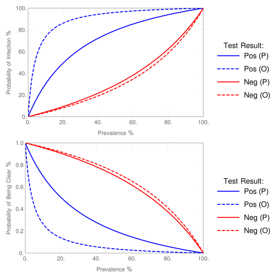
Figure 2: The probability of a correct RT-PCR test result, for both positive and negative test results, vs the prevalence of SARS-CoV-2 in the test pool per 100k population. Two curves are given for each, where (P) indicates a pessimistic 17% false positive rate, and (O) indicates optimistic 2.6% false positive rate. At the time of writing, many western countries are experiencing a prevalence of 0.6% (600 cases per 100k population in a 2 week period).
