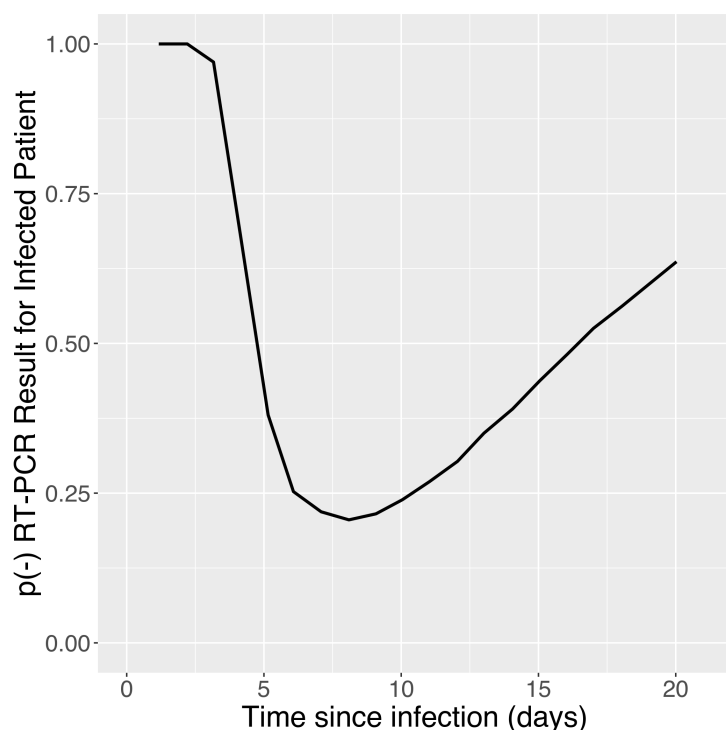
Figure 1: Time dependence of the probability of obtaining a negative RT-PCR result from an infected patient, after Kucirca et al [20].
