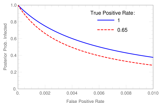
Figure 3: With even a relatively high prevalence of 600 cases per 100k population, these curves show that a false positive rate of < 0.001 is needed for a useful test, i.e. a specificity of > 99.9\% . This result is not strongly affected by the true positive rate, as shown by the two curves indicating a perfect test or with the true positive rate of 0.65 as used in the rest of this paper.
