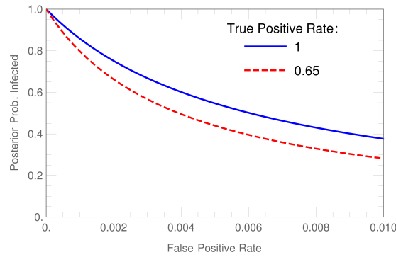
Figure 2: With even a relatively high prevalence of 600 cases per 100k population, these curves show that a false positive rate of < 0.001 is needed for a useful test, i.e. a specificity of > 99.9\% . This result is not strongly affected by the true positive rate, as shown by the two curves indicating a perfect test or with the true positive rate of 0.65 as used in the rest of this paper.
