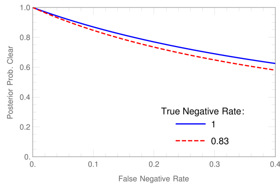
Figure 3: In an extremely high prevalence of 0.6 (60k cases per 100k population) such as in a hospital, jail, or some other sealed outbreak cluster, these curves show that a false negative rate of < 0.05 is needed for a useful test to rule out infection, i.e. a sensitivity of > 95\% . This result is not strongly affected by the specificity, as shown by the two curves indicating a perfect test (specificity = 1) or with the false positive rate of 0.17 (specificity = 0.83) as used in the rest of this paper.
