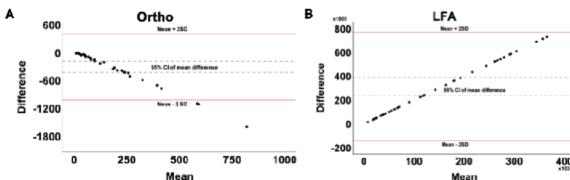
Figure 4. Bland-Altman plots showing bias (mean difference and 95% CI) and computed limits of agreement (mean difference \pm 2SD) between (A) Ortho Vitros Anti-SARS-CoV-2 IgG test and IC 50 values and (B) our LFA and IC 50 values. Thirty-eight samples were tested.
