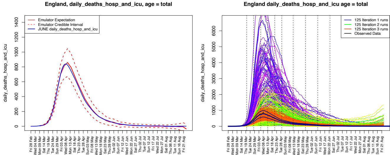
Figure 27: Left Panel: an example diagnostic showing the emulator prediction E_D(f_i(x)) for f_i(x) across several time points (the solid red line) and the prediction interval E_D(f_i(x)) \pm 3\sqrt{\text{Var}_D(f_i(x))} (the red dashed lines) along with the held out smoothed run output f(x) (the blue line). The emulator captures the behaviour of the JUNE model well. Right panel: daily hospital deaths for all of England, showing the progression of the runs from iterations 1, 2 and 3 used in the history matching process (in purple, green and red respectively). Observed data (smoothed and original) in black. Vertical dashed lines: emulated outputs.
