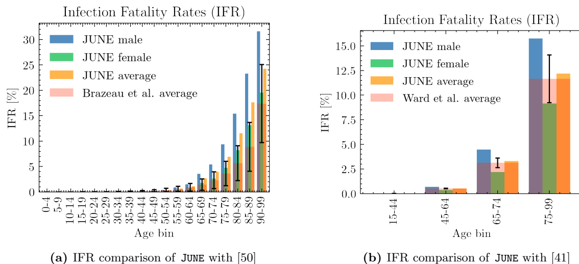
Figure 12: IFR comparison of JUNE with other works.
