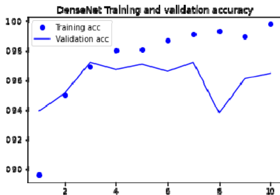
Figure 8. DenseNet accuracy
