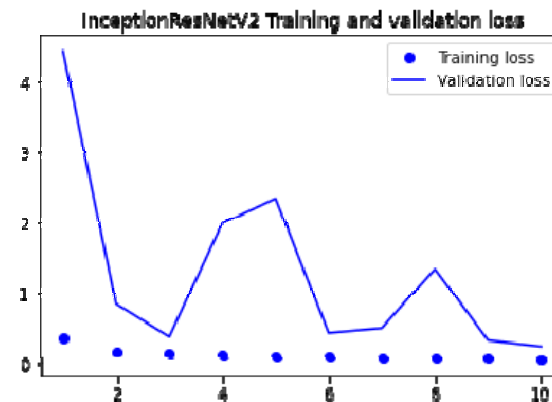
Figure 13. InceptionResNetV2 loss
