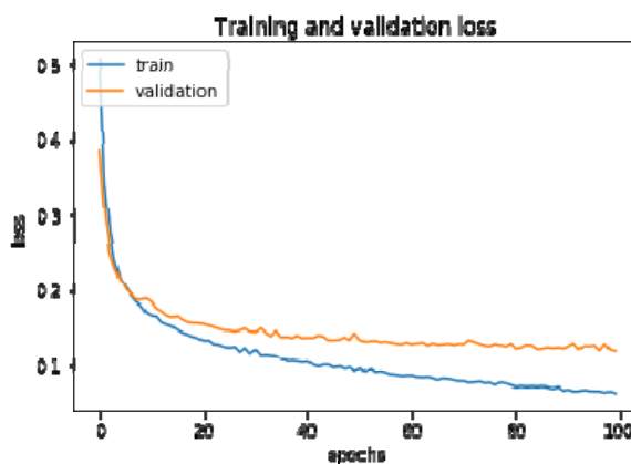
Figure 23.fusion model loss
