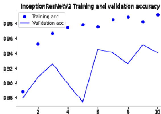
Figure 12. InceptionResNetV2 accuracy
