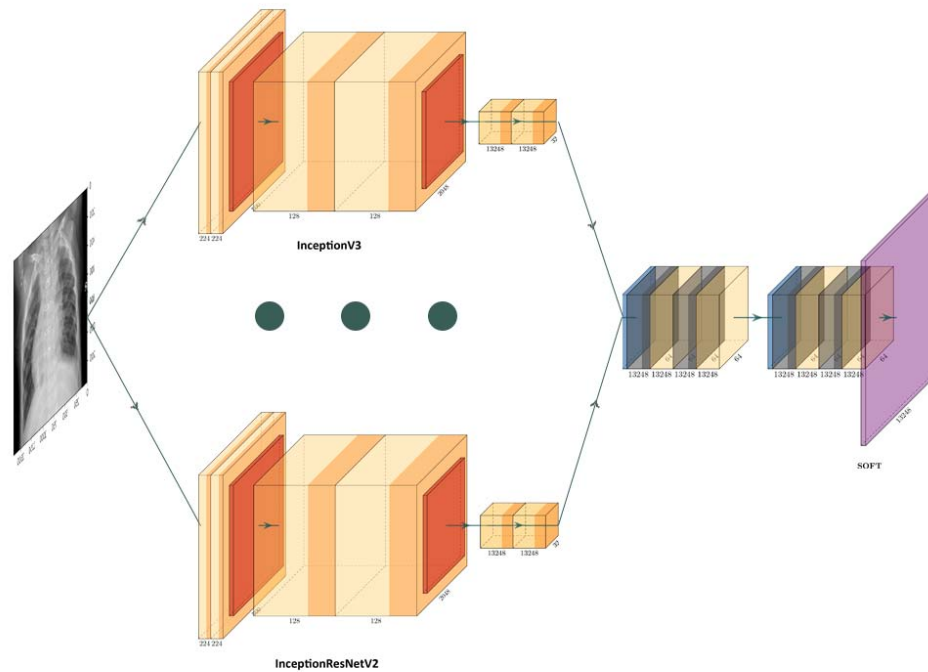
Figure 7.model fusion diagram
