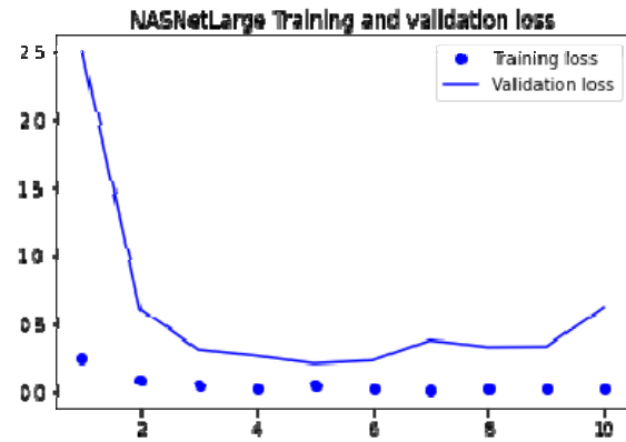
Figure 15.NasLargeNet loss
