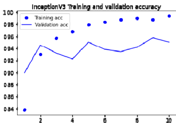
Figure 10. InceptionV3 accuracy
