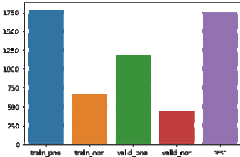
Figure 4.data set distribution
