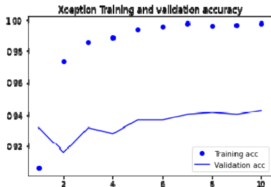
Figure 20.Xception accuracy
