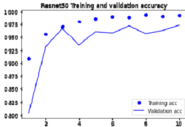
Figure 16.ResNet50 accuracy
