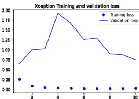
Figure 21.Xception loss
