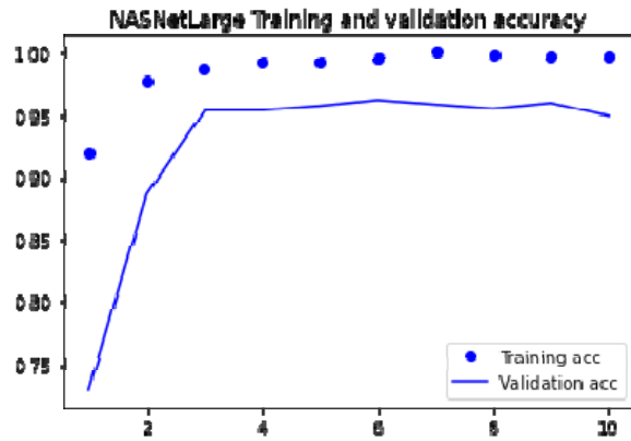
Figure 14.NasLargeNet accuracy
