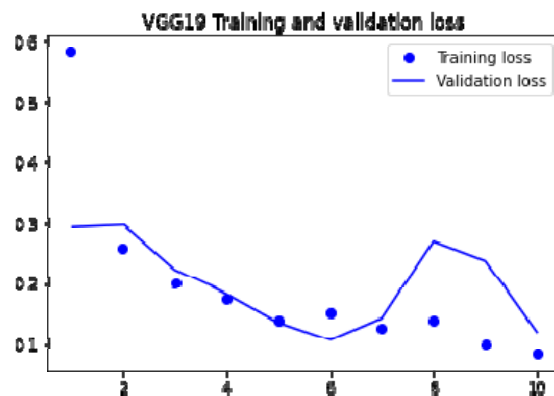
Figure 19.VGG19 loss
