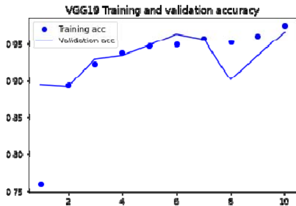
Figure 18.VGG19 accuracy
