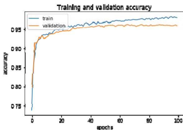
Figure 22.fusion model accuracy
