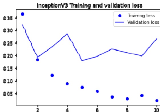
Figure 11. InceptionV3 loss
