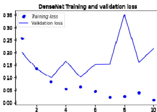
Figure 9. DenseNet loss
