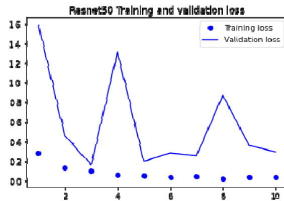
Figure 17.ResNet50 loss
