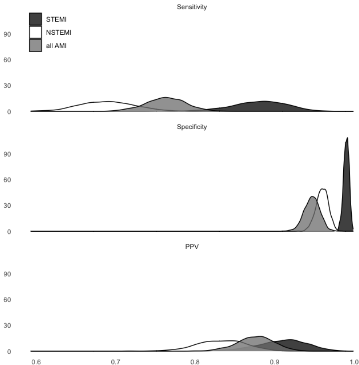
Figure 2. Out-of-sample distributions (density)
