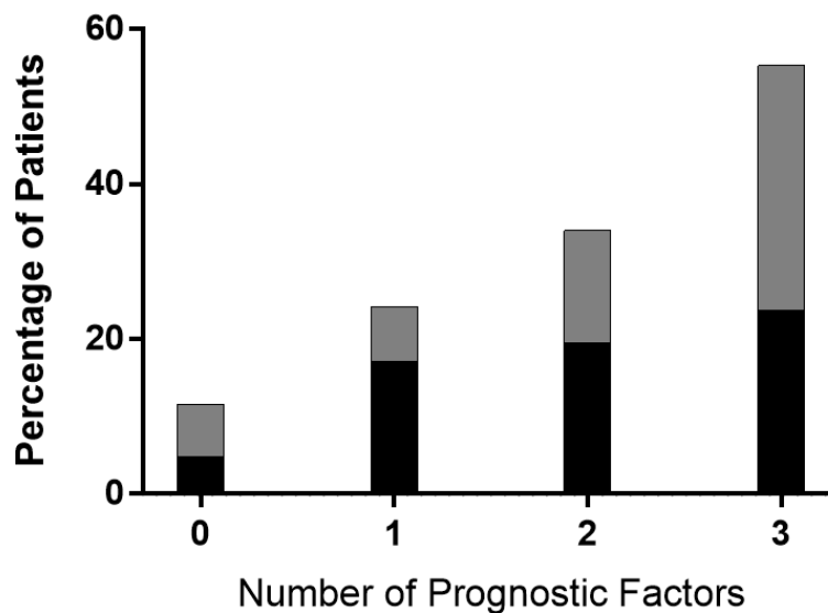
Figure 1. Proportion who relapsed or experienced relapse or 30-day mortality given the number of prognostic factors
