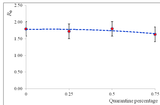
Figure 8: The basic reproductive number as a function of quarantine degree. The dotted line represents a 2 nd degree polynomial fit.
