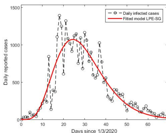
Figure 9: The epidemiological data (DNC) referring to Switzerland at the first phase of epidemic outbreak since 1/3/2020.
