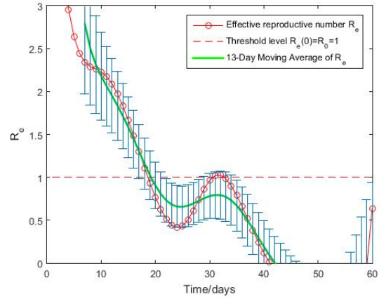
Figure 4: The effective reproductive number as a function of time. The error bars correspond to the moving average values.
