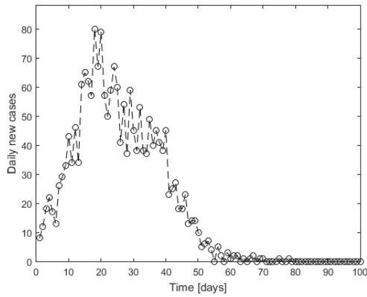
Figure 3: The generated epidemiological data (DNC) from the MC simulation, counted day-by-day along the whole area.
