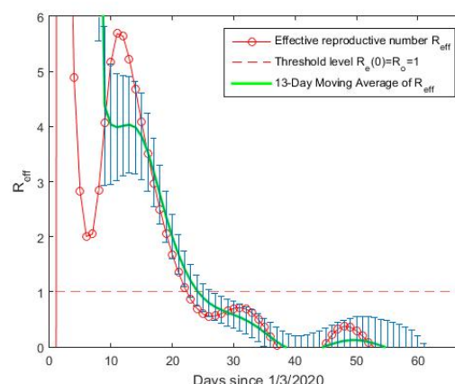
Figure 10: The effective reproductive number as a function of time for the first phase of epidemic outbreak in Switzerland.
