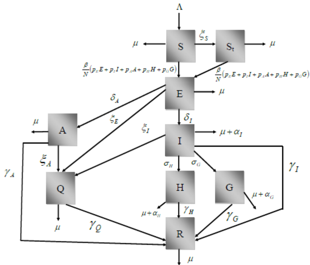
Figure 1 – Schematic representation of the model compartments.
