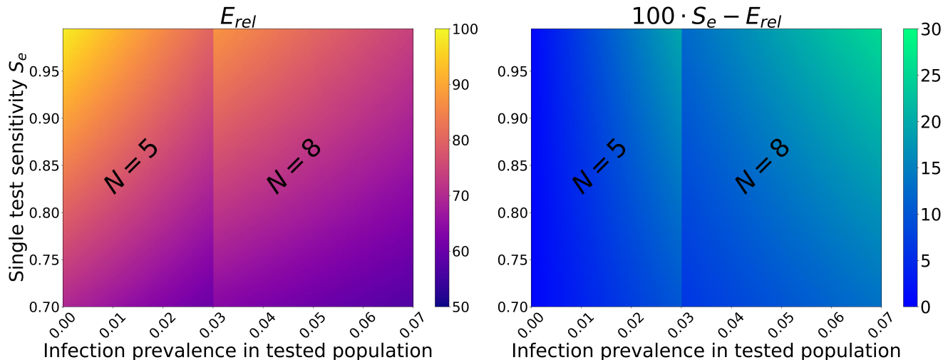
Figure 1: Relative increase in Dorfman pooling false-negative rates E_{rel} . Left: Colors represent E_{rel} , the relative percentage increase in the scheme false-negative rates relative to the single test false-negative rates (eq (3)). Right: colors represent the difference between the approximation assumed in other studies and E_{rel} as calculated by our model. The disease prevalence q , is varied on the x-axis, while the test sensitivity is varied on the y-axis. Pool size N , was chosen according to q as in [2].
