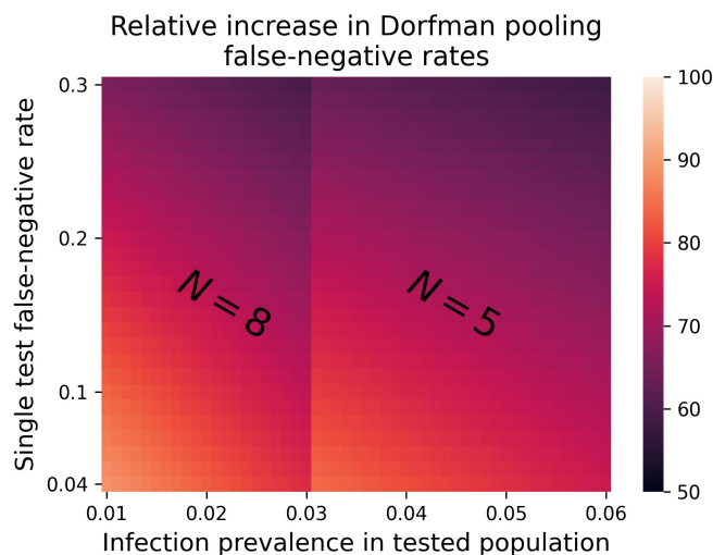
Figure 1: Relative increase in Dorfman pooling false-negative rates E_{rel} . Color represents the relative percentage increase in the scheme false-negative rates relative to the single test false-negative rates, P_{fn} . The disease prevalence, q , is varied on the x-axis, while the single test false-negative rate is varied on the y-axis. Note that Pool size, N , was chosen according to q as in [1].
