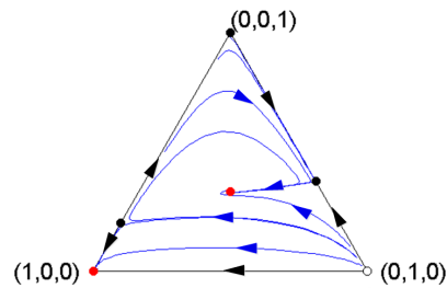
Figure 2: Trajectories of the game with an attractor not coinciding with an ESS, depicted in the simplex. The vertices correspond to populations consisting of just one type. Example from [175].
