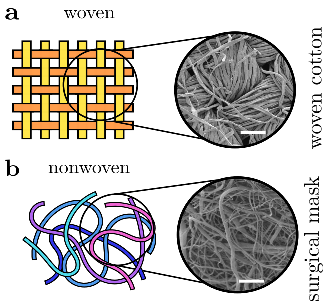
FIG. 2. Fabrics are broadly categorised as knitted (not shown), woven or non-woven . (a) Woven fabrics formed by intersecting perpendicular yarns (the “warp” and “weft”). (b) Nonwoven fabrics are formed by entangling fibres through other means, resulting in less ordered arrangements. Scanning electron microscope images of example fabrics show scalebars of (a) 100 \mu\text{m} and (b) 50 \mu\text{m} .
