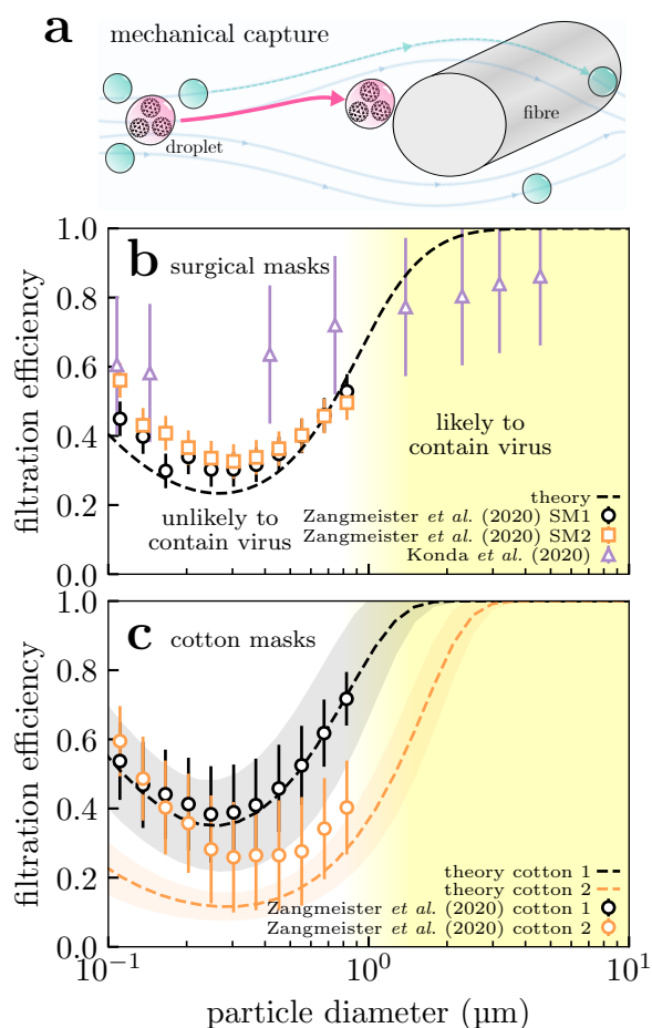
FIG. 1. Variation in mask filtration efficiency with incoming particle size. (a) Diagram of capture of viral particles by a fibre within a mask. Larger particles are more easily captured because they are less mobile; smaller aerosols by contrast are transported around the fibre by the gas flow. Larger particles can also carry more virions, and submicron aerosols are unlikely to contain even a single virion (cf. text). The filtration efficiency of perfectly fitting (b) surgical masks and (c) cloth masks formed from 4 identical plain-woven cotton layers are shown as a function of particle size. We show experimental measurements from Refs. 33 and 34 (points) and predictions from our model (lines) which is described elsewhere 35 and the Supplementary Material. The shaded envelopes around the lines in (c) show the uncertainty in the model predictions, obtained by propagating uncertainties in the geometric parameters given in Ref. 34. We set the velocity of the gas through the mask to 6.3 \text{ cm s}^{-1} in our calculations for comparison with data from Ref. 34.
