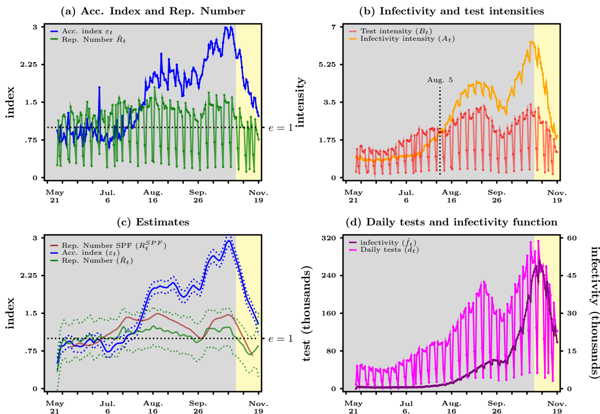
Figure 3: France - Panel (a) Acceleration index (blue curve) vs reproduction number (green curve). Panel (b) Infectivity intensity (orange curve) vs test intensity (red curve). Panel (c) Kernel estimates with confidence bands (dashed lines). Panel (d) Daily tests (purple line) and infectivity function (black curve). Beige area depicts the lock-down period. Source: Agence Santé Publique France and authors' computations.
