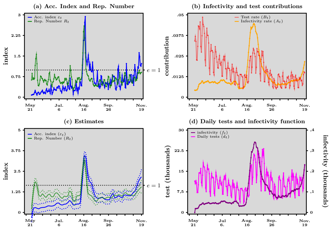
Figure 7: South Korea - Panel (a) Acceleration index (blue curve) vs reproduction number (green curve). Panel (b) Infectivity contribution (orange curve) vs test contribution (red curve). Panel (c) Kernel estimates with confidence bands (dashed lines). Panel (d) Daily tests (purple line) and infectivity function (black curve). Source: Our World in Data and authors' computations. Testing data for South Korea were incomplete: five dates were missing. Missing values were completed by a linear interpolation.
