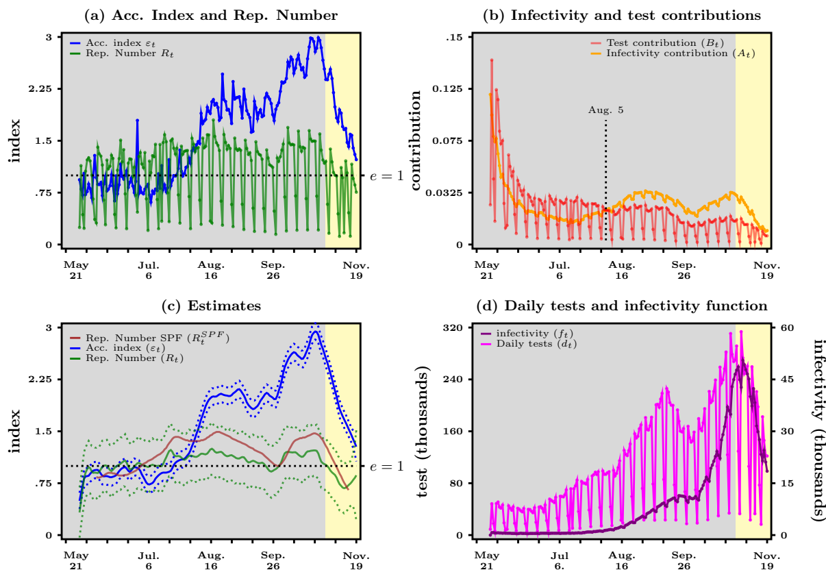
Figure 2: France - Panel (a) Acceleration index (blue curve) vs reproduction number (green curve). Panel (b) Infectivity contribution (orange curve) vs test contribution (red curve). Panel (c) Kernel estimates with confidence bands (dashed lines). Panel (d) Daily tests (purple line) and infectivity function (black curve). Beige area depicts the lock-down period. Source: Agence Santé Publique France and authors' computations.
