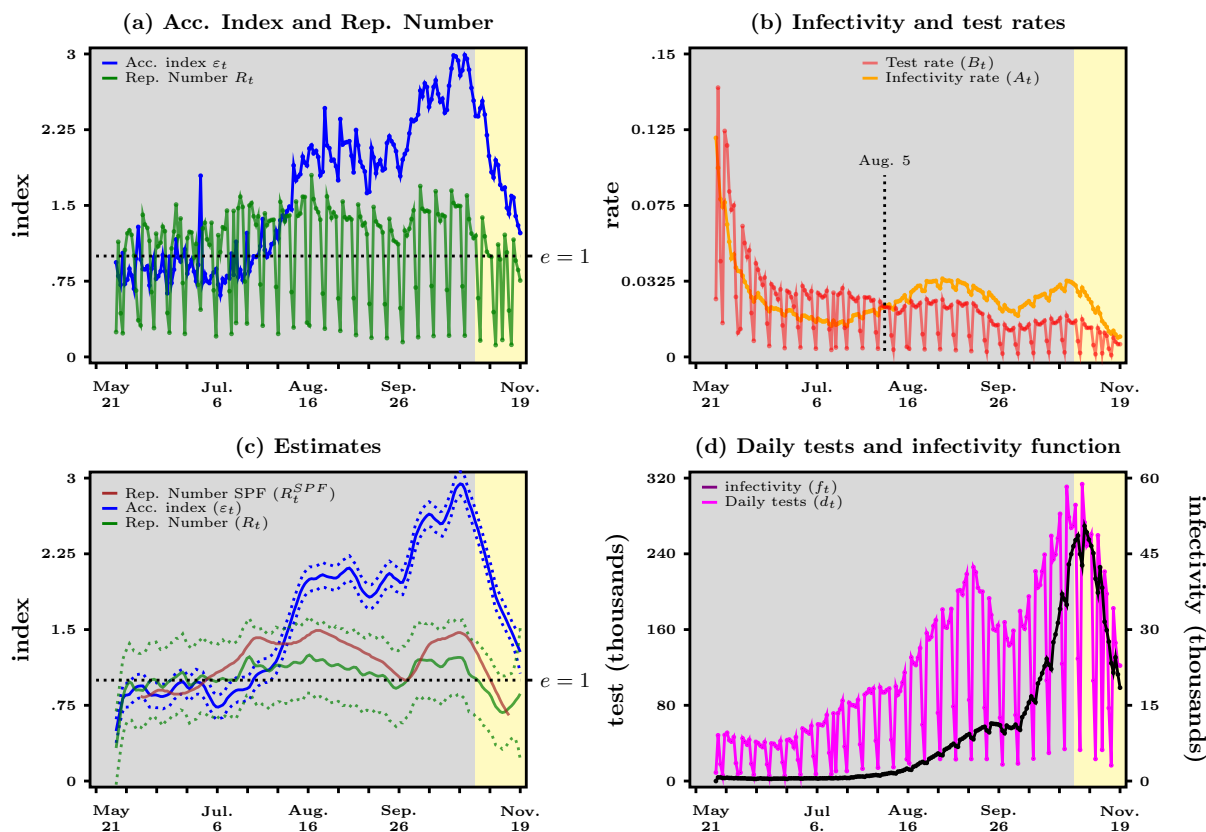
Figure 2: Panel (a) Acceleration index (blue curve) vs reproduction number (green curve). Panel (b) Infectivity rate (orange curve) vs test rate (red curve). Panel (c) Kernel estimates with confidence bands (dashed lines). Panel (d) Daily tests (purple line) and infectivity function (black curve). Beige area depicts the lock-down period. Source: Agence Santé Publique France and authors' computations.
