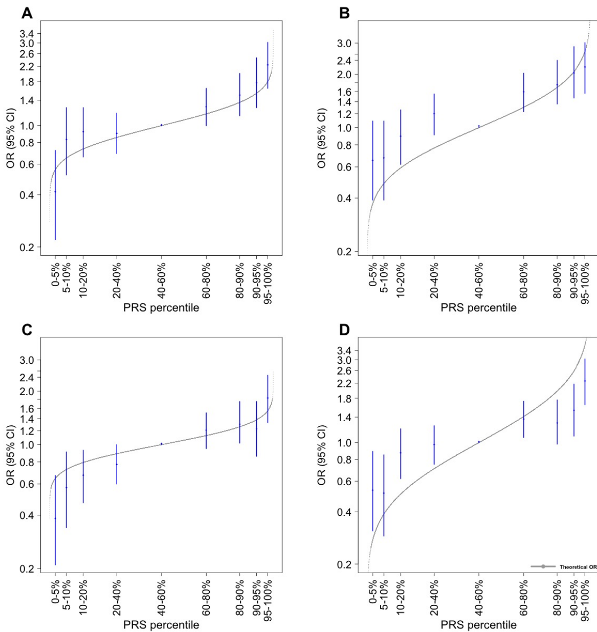
Figure 3: Association between the PLR PRS models and non-mucinous ovarian cancer by PRS percentiles
