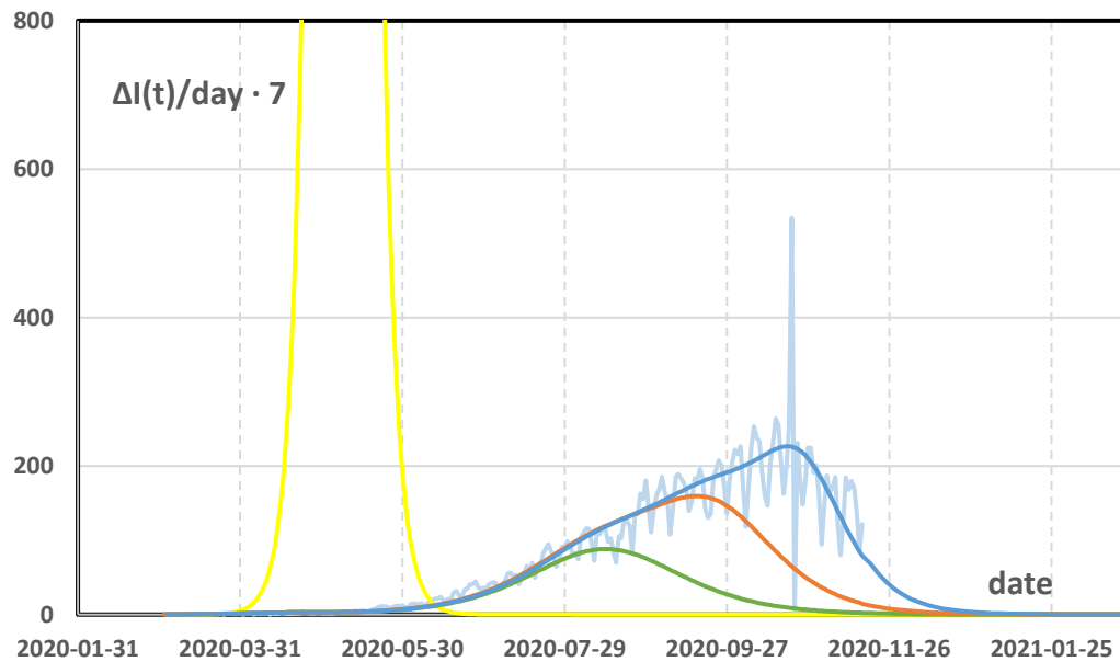
Figure 2: Infection rate per 100,000 persons per week. The vertical axis directly compares with the numbers for incidences per 100,000 persons per week as used e.g. for identifying high risk regions. Light blue: observed infection rates with strong weekly oscillations, colors for fitted outbreaks as in Figure 1. All infection rates were calculated from the respective data for total case numbers by taking the day-by-day differences and multiplying by seven.
