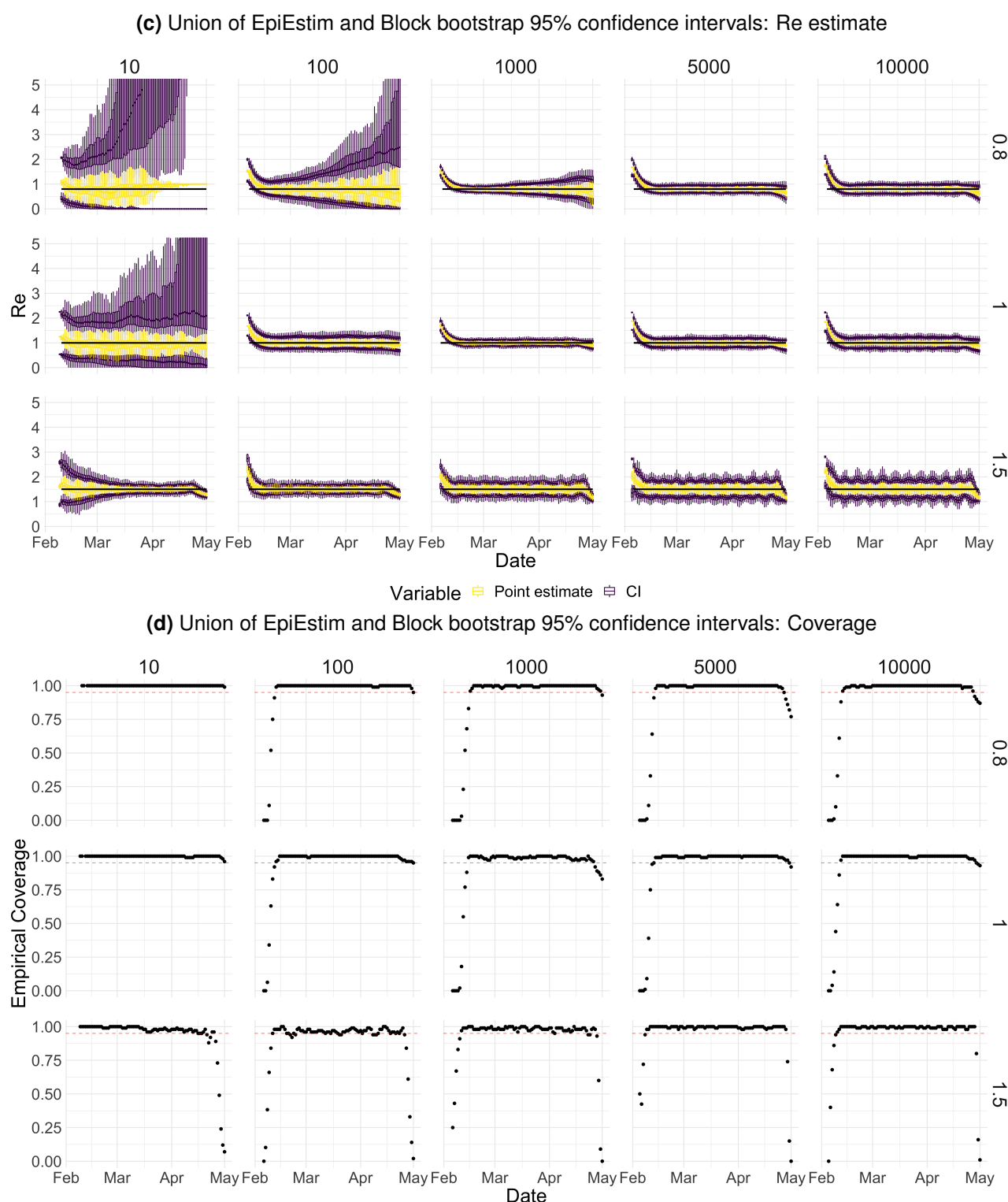
Figure S5: Performance of our method on simulated scenarios with varying population size. (a), (c) We specified a constant R_e \in \{0.8, 1, 1.5\} value (black line; rows) to simulate a trajectory of reported cases (with Swiss case observation noise) 100 times. From each trajectory we estimated R_e (yellow boxplots), and constructed a 95% confidence interval (purple boxplots of the lower/upper endpoint). The simulated scenarios had differing initial incidence of I_0 \in \{10, 100, 1000, 5000, 10000\} infections per day (columns). In the top row, R_e < 1 so the epidemic is decreasing. In the middle row, R_e = 1 , the epidemic is constant, and in the bottom row, R_e > 1 , the epidemic is increasing. The bias at the start is due to the initialisation of the simulation. (b), (d) The fraction of simulations where the true R_e value was within the 95% confidence interval. The dashed red line indicates the nominal 95% coverage. We see that for a wide range of infection incidences, our 95% confidence interval is informative and covers the true value of R_e , whereas the EpiEstim coverage strongly declines with increased epidemic size.
