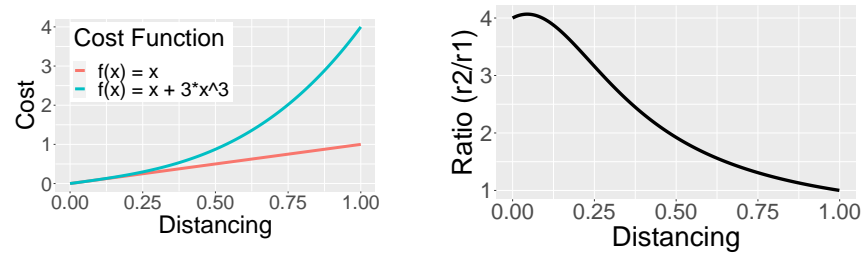
Figure 1: The two isolation cost functions (left) differ by a modest ratio in their risk thresholds ( r_2/r_1 ; right) as a function of population-wide distancing.
