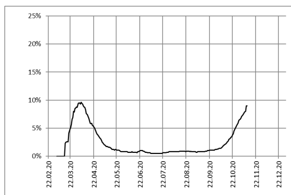
Fig. 3. Positive rate [6]
