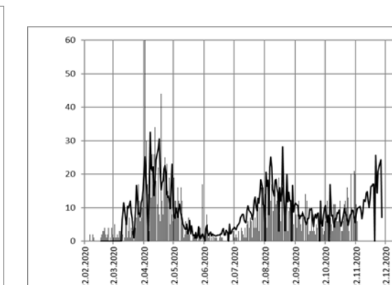
Fig. 16. JPN: IFR = 3 per million inhabitants
