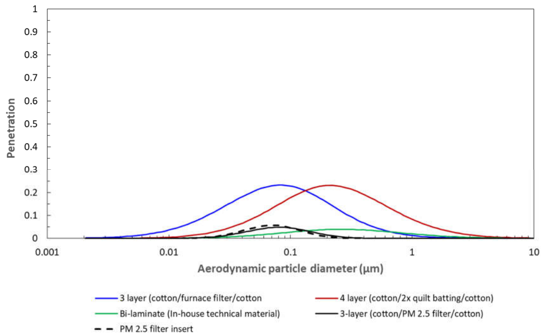
Figure 5: Penetration profile as a function of aerodynamic particle diameter for four multi-layer material systems that may be used in reusable cloth face coverings. Solid lines are the merged log-normal composite distribution curve-fit obtained from the actual measured SMPS and APS data. A penetration value of 1 equates to 100% of aerosol penetrating through the material. The aerosol penetration through only the PM 2.5 filter insert is shown separately as a dashed line.
