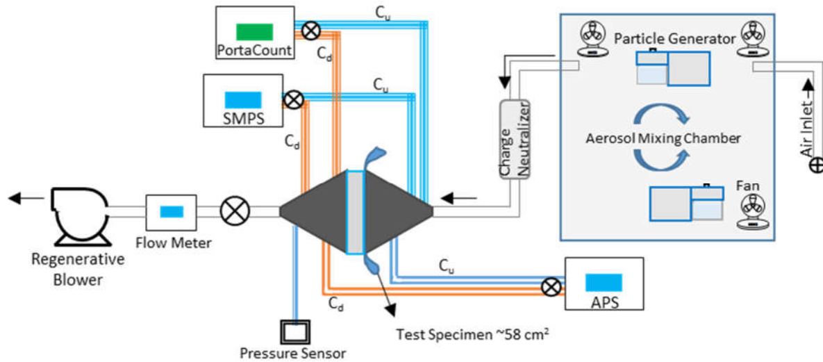
Figure 1: Schematic of aerosol switch penetration set-up. A polydisperse NaCl aerosol is generated in the mixing chamber and pulled through the charge neutralizer and switch test rig using a regenerative blower. Air flow is regulated using the flow meter. Aerosol concentration, upstream and downstream, is measured with the SMPS/APS and PortaCount as shown.
