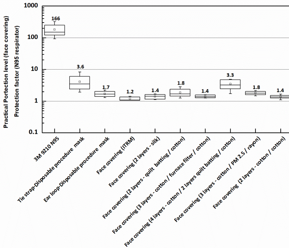
Figure 7: Practical protection level obtained for the various reusable cloth face coverings compared to the practical protection level for two different styles of disposable procedure mask and the protection factor obtained for a N95 FFR. The number shown above the marker denotes the geometric mean, also indicated by the small square marker; the line inside the box is the median, the upper and lower limit of the box are the 25 th and 75 th percentiles, and; the whiskers are the minimum and maximum values measured. The sample size for the N95 FFR, the disposable procedure mask with ear loops (Henan Liwei) and the reusable 2 layer cotton homemade face covering (CC) was n=8 . For all other face coverings the sample size was n=5 .
