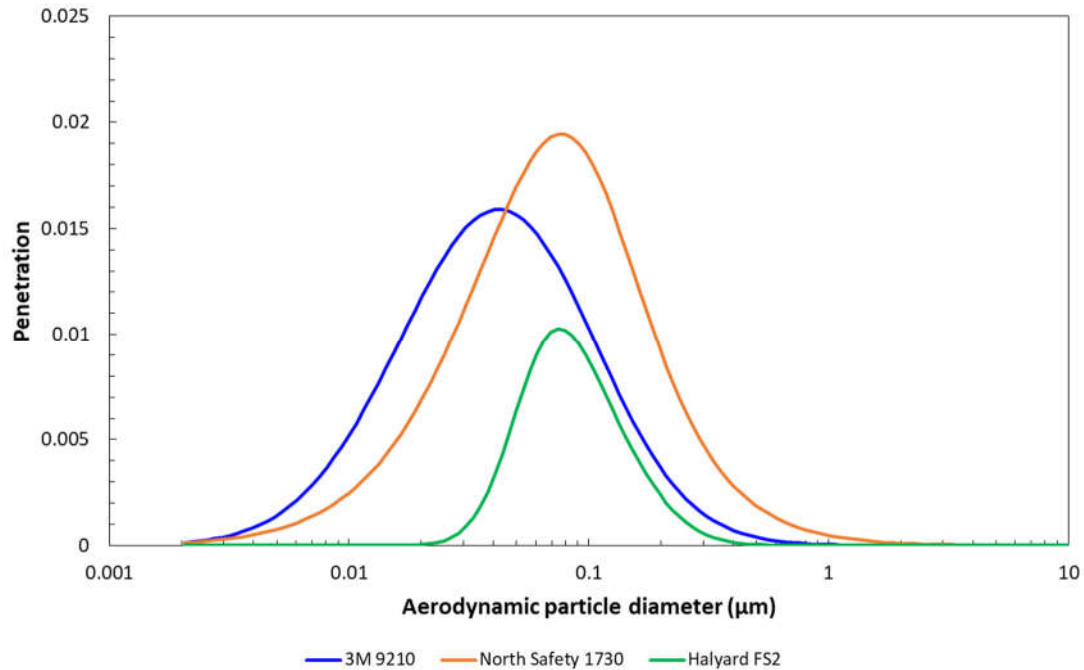
Figure 3: Penetration profile as a function of aerodynamic particle diameter for the filter material of three N95 FFRs. The curves shown are the merged log-normal composite distribution curve-fit obtained from the SMPS and APS data. Aerosol penetration was collected at a nominal flow rate of 17 L/min. Note the y-axis scale maximum is 0.025. A penetration value of 0.025 equates to 2.5% of aerosol penetrating through the material.
