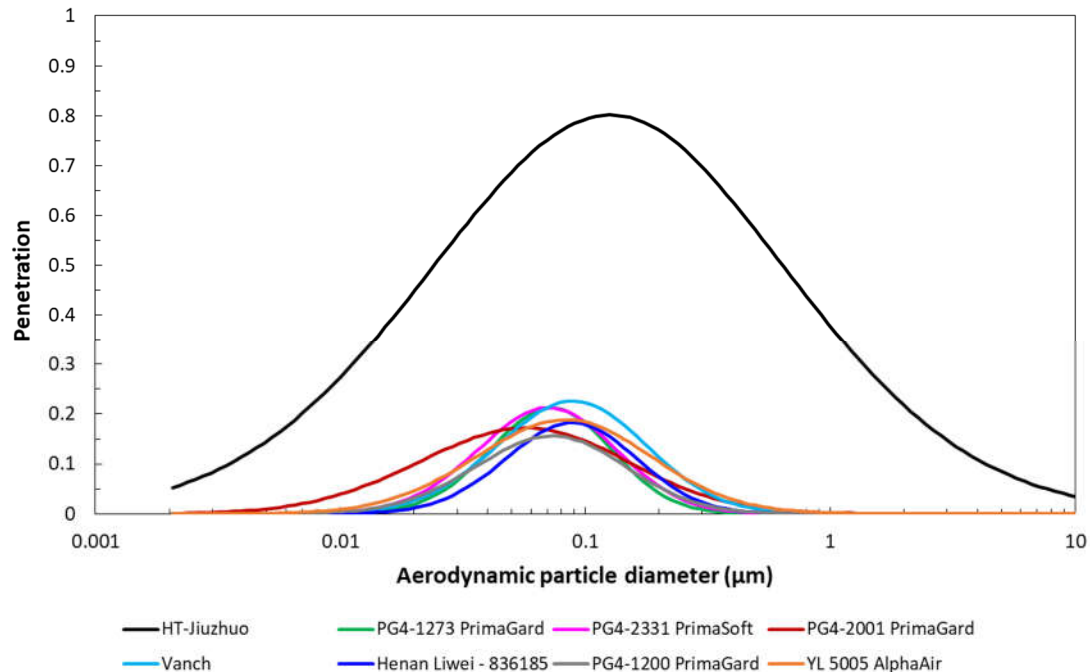
Figure 6: Penetration profile as a function of aerodynamic particle diameter for eight disposable procedure mask material systems. Solid lines are the merged log-normal composite distribution curve-fit obtained from the actual measured SMPS and APS data. A penetration value of 1 equates to 100% of aerosol penetrating through the material.
