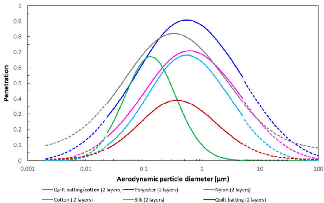
Figure 4: Penetration profile as a function of aerodynamic particle diameter for common fabrics used in reusable cloth face coverings. The solid segment of the curves are the merged log-normal composite distribution curve-fit obtained from the actual measured SMPS and APS data. Dashed lines show extrapolated penetration values for the particle size distribution beyond the experimental measurement range of 0.023 to 5.0 \mu\text{m} investigated. A penetration value of 1 equates to 100% of aerosol penetrating through the material.
