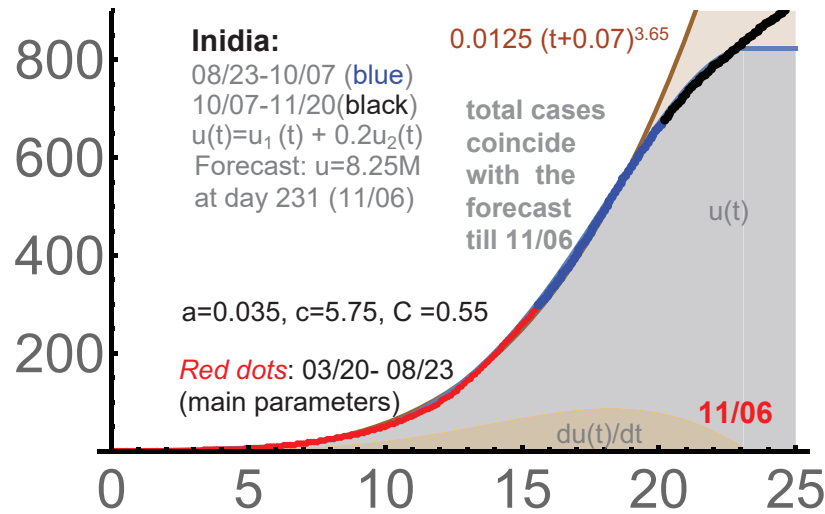
FIGURE 1. India: 3/20-10/7, c=5.75 , a=0.035 , C=0.55 .
