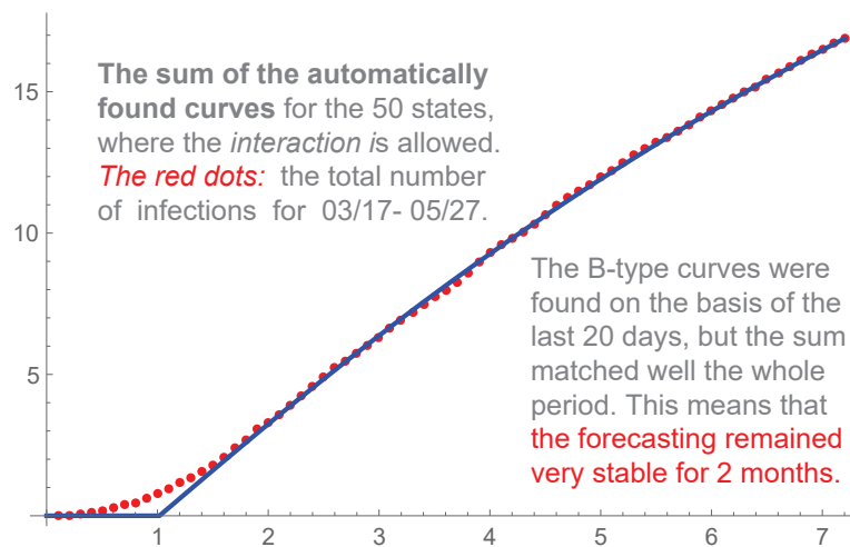
FIGURE 11. USA, the sum of the curves for individual states.
