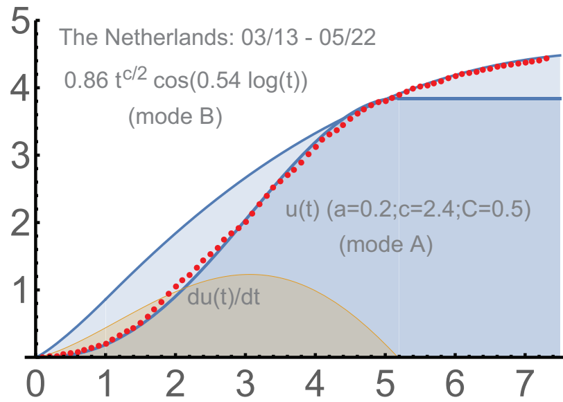
FIGURE 5. The Netherlands: u = 0.5t^{1.7} J_{0.7}(t\sqrt{0.2}) .
