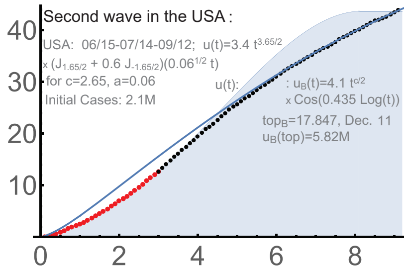
FIGURE 7. 2-phase solution for the 2nd wave in the USA.
