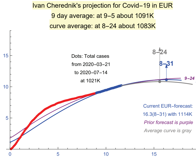
FIGURE 12. A sample auto-forecast for Europe as of 7/14.
