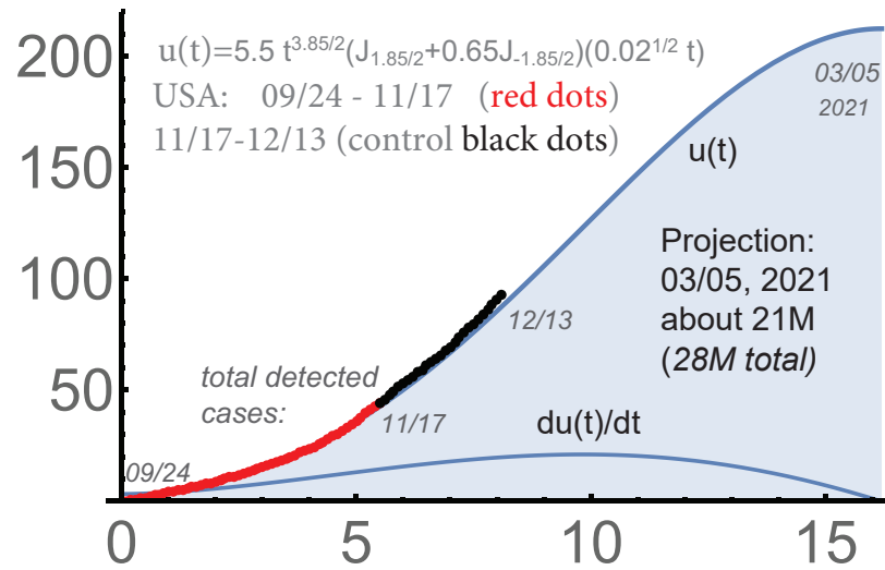
FIGURE 9. The 3rd wave in the USA.
