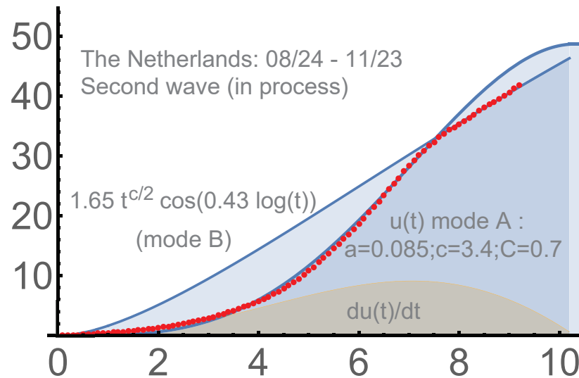
FIGURE 10. The 2nd wave in the Netherlands.
