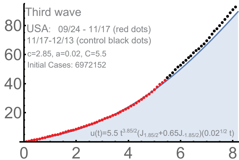
FIGURE 8. The 3rd wave in the USA.
