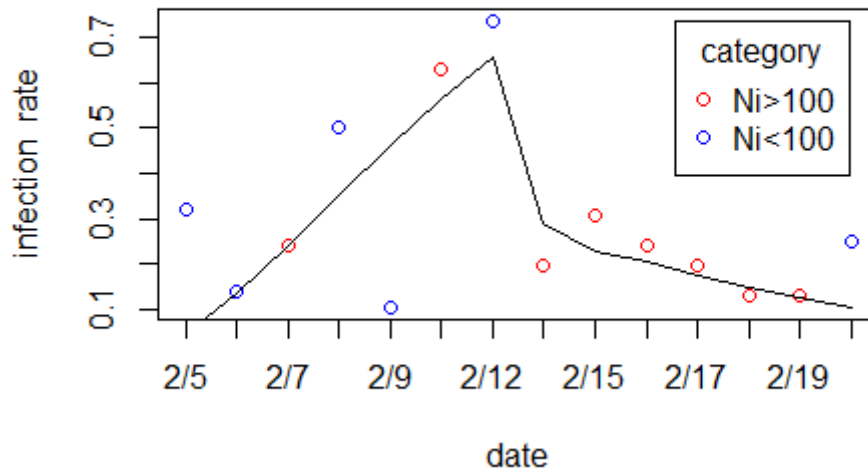
Figure 3: Comparison of n_i/N_i and fitted weibull infection distribution. n_i represents daily number of positive individuals, and N_i is the total number of tests each day. Scatter points are the rate of n_i/N_i . Black line shows the fitted infection distribution consisting of \lambda_i F_i .
