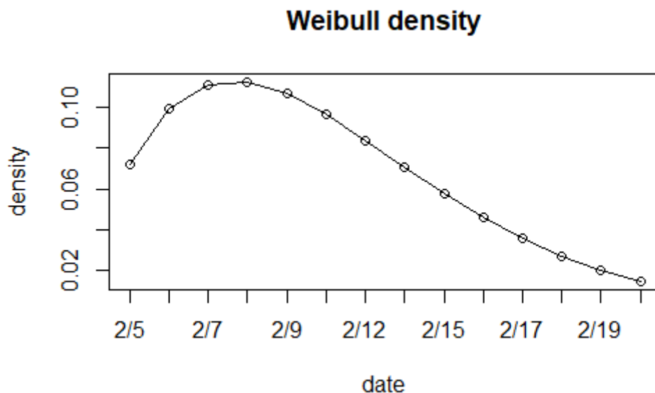
Figure 2: Fitted Weibull density function of infection time
