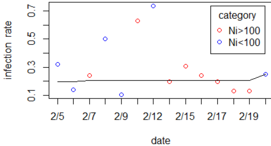
Figure 1: Comparison of \mathbf{n}_i/\mathbf{N}_i and fitted infection rates using PAVA. n_i represents daily number of positive individuals, N_i is the total number of tests each day. Scatter points are the rate of n_i/N_i . Blue points represent those whose corresponding total test number was less than 100, while red points mean the total test number was larger than 100. Black line shows the fitted infection distribution consisting of F_i .
