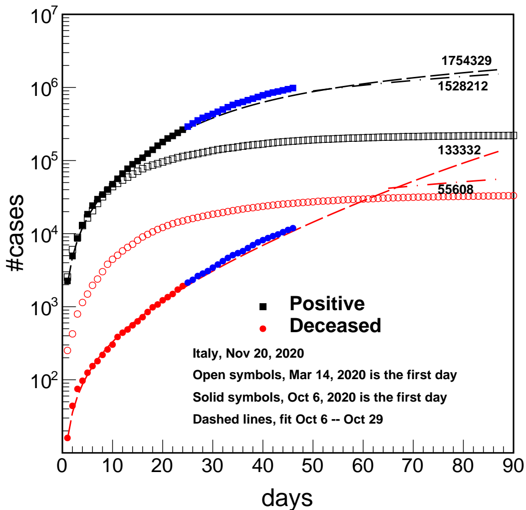
Fig. 1. (Color online) Number of cases vs. time in days in Italy. The open symbols refer to the effective data registered starting from March 14 th , 2020: the lockdown day. The full symbols refer to data starting from October 6 th . The dashed lines are from the fits, eqs. (1-3).
