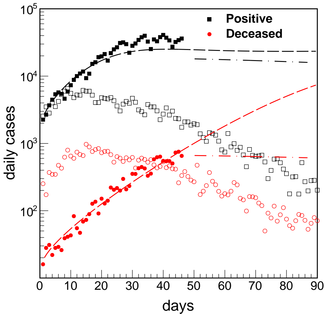
Fig. 3. (Color online) Number of daily cases vs time, symbols as in figure 1. This quantity can be obtained from the time derivative of the quantities reported in figure 1 or from data directly (open and full symbols).
