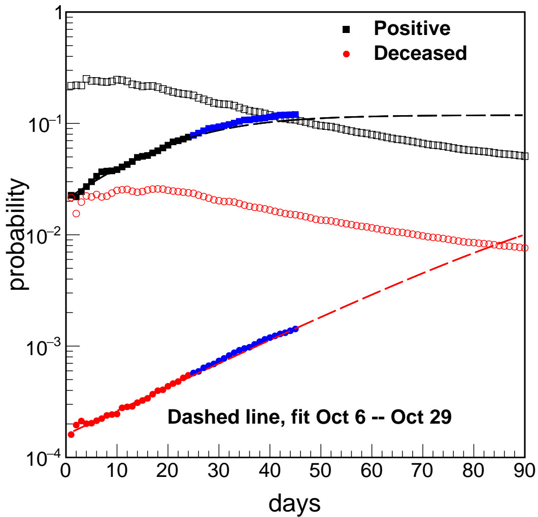
Fig. 2. (Color online) Same as figure 1 but for the probabilities given by the number of cases divided the number of tests [1]. Fits are obtained using eq. (1), no decay stage is observed yet, opposite to the Spring data (open symbols).
