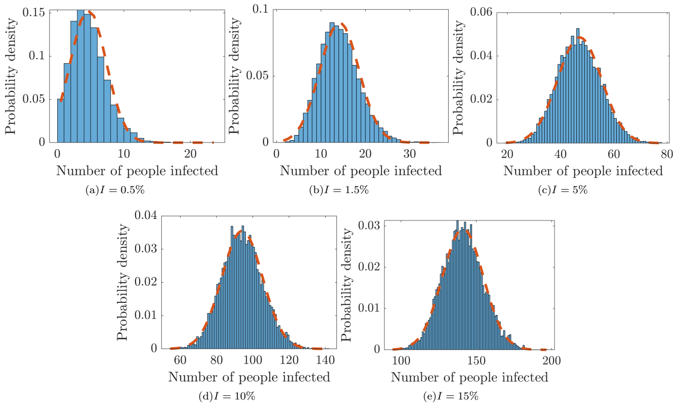
FIG. 2: Histogram and data fit representing the variability over 10^4 Monte-Carlo simulations. The blue histogram is the simulated data, the red dashed line is the fit of a normal distribution. Note that we are plotting the probability density, but since each column is one person wide the y values can be interpreted as a probability.
