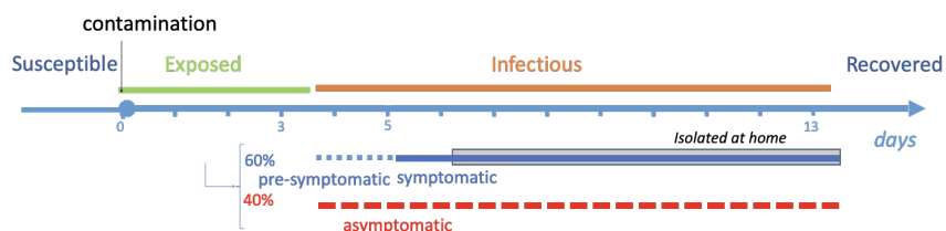
Figure 2: The infection model for SARS-Cov2. The incubation (Exposed, green) lasts on average 3.7 days and is followed by an infectious period (Infectious, orange) of mean 9.5 days. For symptomatic patients, symptoms appear 1.5 days after the beginning of infectiousness on average, and we assume that those patients self-isolate after one day of symptoms. Asymptomatic individuals do not isolate.
