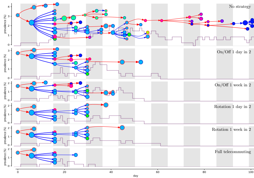
Figure 5: Epidemic propagation in the contact graph of a highschool, under different strategies: each panel corresponds to an example simulation for a given strategy; strategies are sorted as by effectiveness (according to our three metrics), from none (business as usual) to full telecommuting. In each panel, the horizontal axis corresponds to time (in days), and each white or gray column corresponds to one week. The vertical axis shows the prevalence (percentage of infectious persons in the workplace): its evolution is represented by the grey curves in the background. For each strategy, the epidemic propagation over the contact graph is shown as a tree, where each node represents an infected person and points to the persons it infects. Nodes corresponding to symptomatic (resp. asymptomatic) persons are circled in blue (resp. red). Similarly a blue (resp. red) arrow corresponds to a contamination by a symptomatic (resp. an asymptomatic) person. The thickness of arrows indicates the super-spreading factor. The node color corresponds to the group of the person (class in the case of schools). All the propagation trees are generated using the same realizations of the probabilistic events, so that the differences between the trees are not artifacts of their randomness, but solely depend on the different strategies in place.
