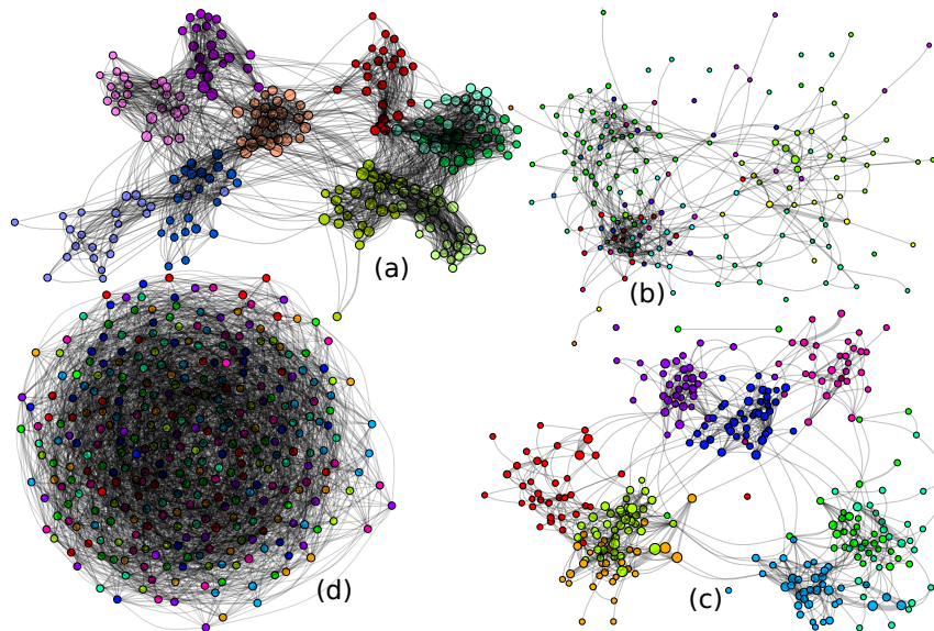
Figure 1: Contact graphs. (a-c) Three contact networks on their busiest day: (a) on day 2, primary school with 242 students, (b) on day 1, workplace with 217 workers, (c) on day 2, high school with 327 students. Node colors correspond to known groups (classes or department). We see that the majority of contacts happen within the same groups. (d) A synthetic random graph with 9 groups selected randomly. For better visualization, in the four graphs only edges representing at least 3 contacts are drawn.
