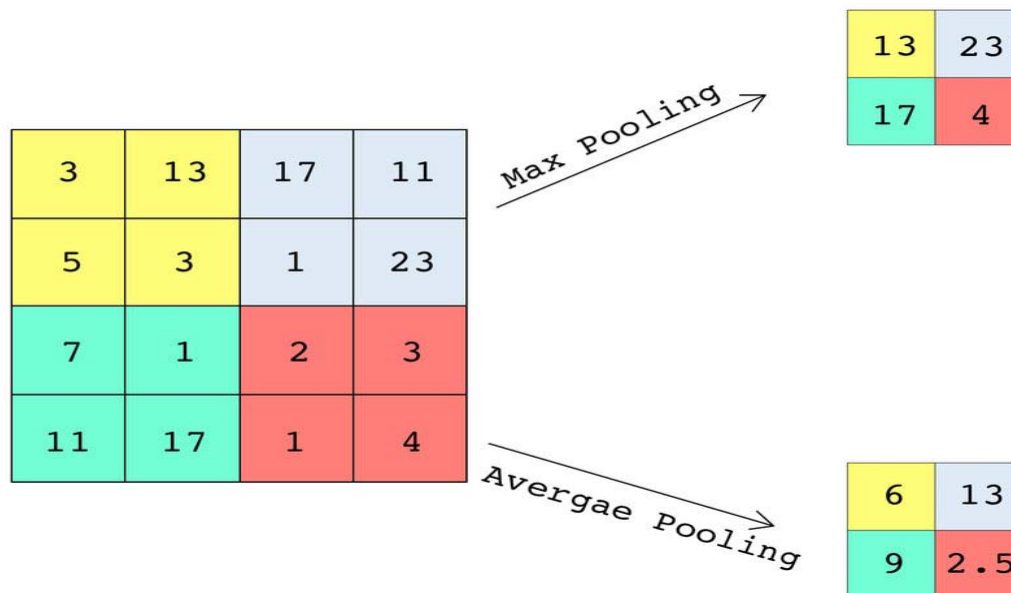
Fig. 3: Example of Max and Average Pooling.
