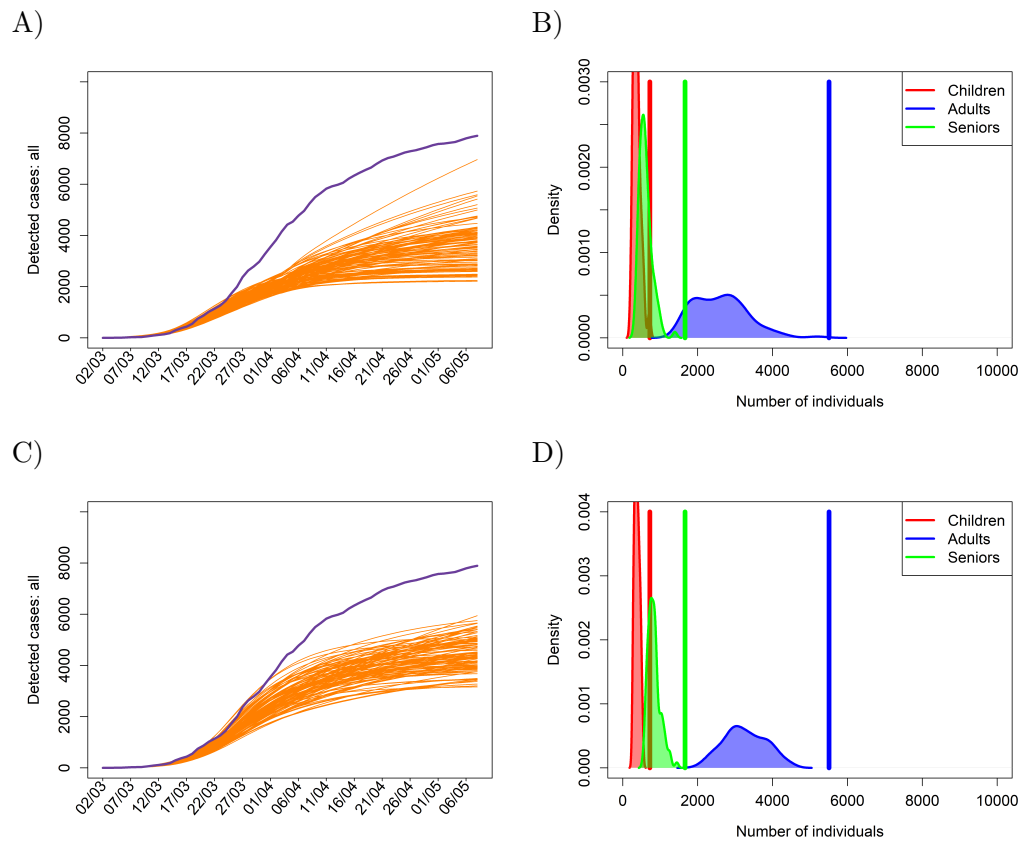
Figure 7: Some other plausible scenarios. Temporal dynamics of the total cumulative numbers of confirmed cases for (A) the scenario with swapped application of personal protective measures (from March 19 to March 11) and closing schools and recommending home office (from March 11 to March 19) or (B) with testing efficiency (average time delay from symptom onset to case confirmation) in March equal to that in April and May. Legend as in Fig. 4.
