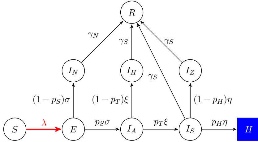
Figure 10: A scheme showing structure of the epidemic and testing model layers. The box H representing hospitalized individuals is elaborated in this section.
