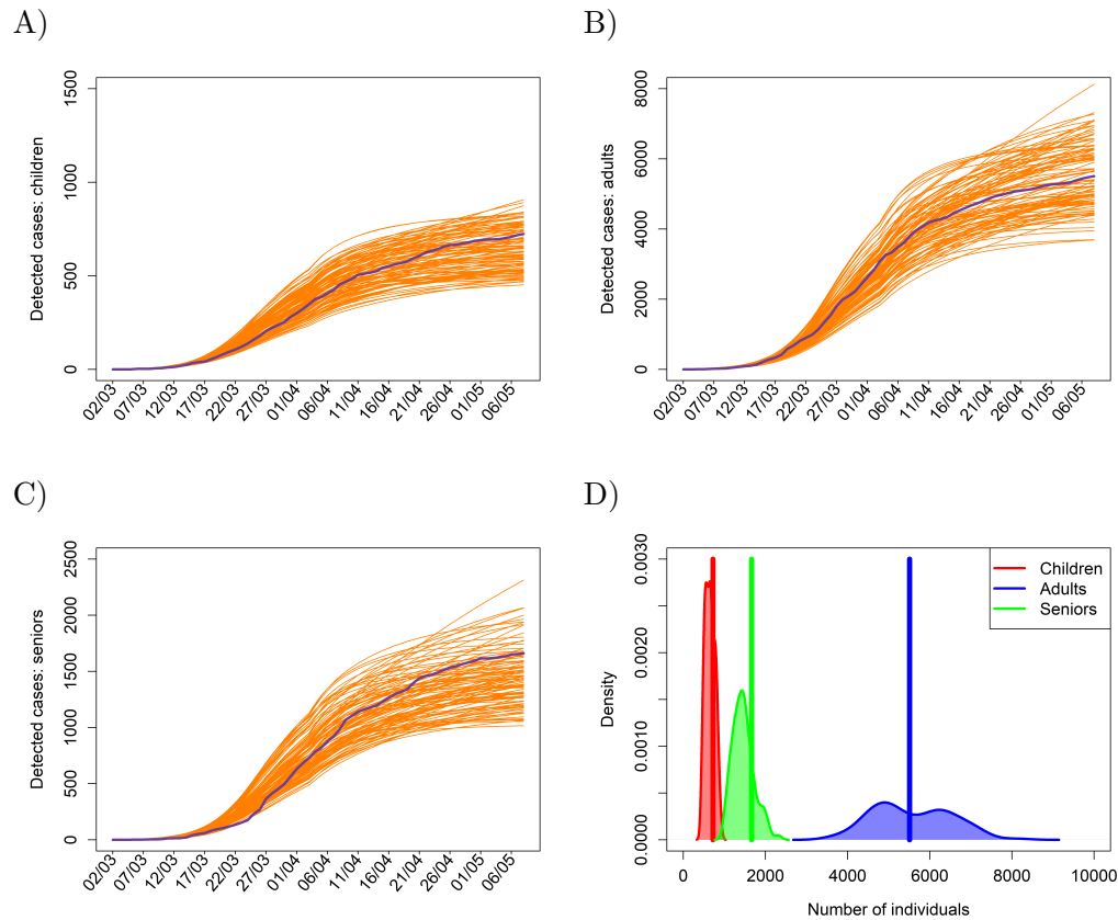
Figure 3: Baseline scenario. Temporal dynamics of the age-structured and total cumulative numbers of confirmed cases for the baseline scenario, covering the initial phase of epidemic and the following lockdown, for children (age cohort 0-19, A), adults (age cohort 20-64, B), seniors (age cohort 65+, C), and the probability density functions for the number of confirmed cases by 7 May 2020 (D). In panels A-C, blue curves represent real observations, while the orange lines are results of model simulations run for 100 selected posterior parameter sets. In panel D, the vertical lines represent the numbers of confirmed individuals by May 7, 2020.
