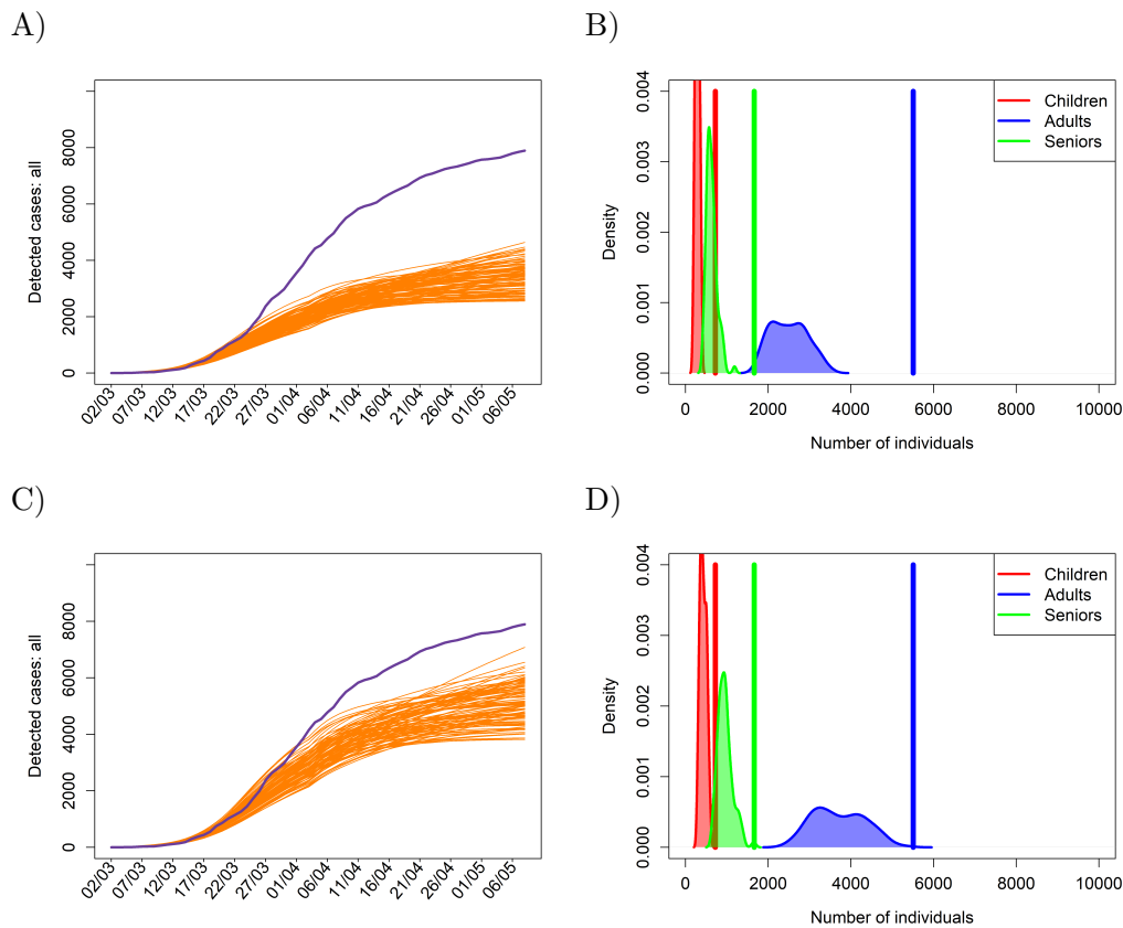
Figure 4: Lockdown scenario shifted backward in time. Temporal dynamics of the total cumulative numbers of confirmed cases for the lockdown scenario shifted four days back (A-B) or two days back (C-D). Blue lines in the left panels represent real observations, while the orange lines are results of model simulations run for 100 selected posterior sets. In the right panel, probability density functions for the number of confirmed cases by 7 May 2020 is provided for each considered age group; the vertical lines represent the numbers of confirmed individuals by May 7, 2020.
