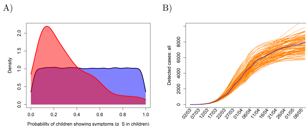
Figure 2: Approximate Bayesian Computation (ABC) . (A) Prior parameter distributions based on available information are first built for every parameter to be estimated (blue distribution). (B) Parameter sets randomly generated from these priors are then used to run the model, and the sets for which the corresponding simulations provided a sufficiently good fit to the observed data were not rejected and were used to build posterior distributions for the estimated parameters; red distribution of panel A is the marginal distributions calculated from the resulting multidimensional posterior distribution.
