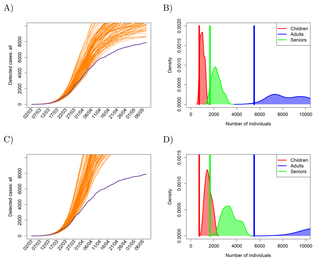
Figure 5: Lockdown scenario shifted forward in time. Temporal dynamics of the total cumulative numbers of confirmed cases for the lockdown scenario shifted two days forward (A-B) or four days forward (C-D). Legend as in Fig. 4.
