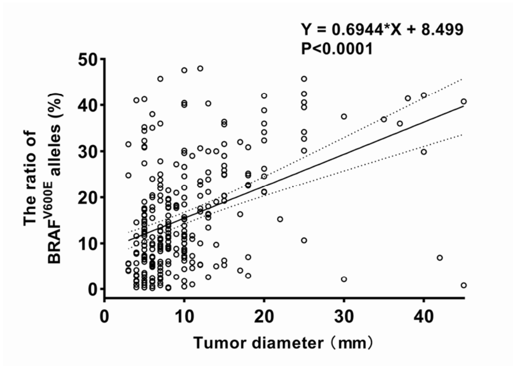
Figure 2. Correlation between BRAFV600E alleles ratio and maximal tumor diameter in PTC. Note: Scatter plot shows the correlation of the ratio of BRAFV600E alleles and tumor diameter. Lines represent simple linear regression \pm 95\% confidence interval. Spearman's rho = 0.413, p < 0.0001 ; simple regression adjusted R^2 = 0.189 , p < 0.0001 .
