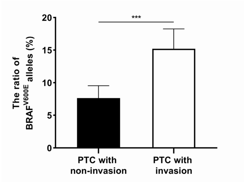
Figure 3. Comparison of BRAFV600E alleles ratio between capsule/extrathyroidal invasion and those without in PTC. Note: ***: P value <0.001; The top of columns represents the median, and lines represent \pm 95 % confidence interval.
