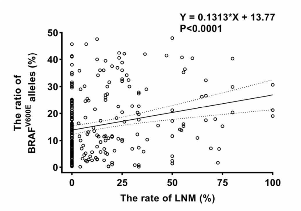
Figure 5. Correlation between BRAFV600E alleles ratio and the rate of lymph node metastases in PTC. Note: Scatter plot shows the correlation of the ratio of BRAFV600E alleles and the rate of LNM. Lines represent simple linear regression \pm 95\% confidence interval. Spearman's rho = 0.232, p < 0.0001 ; simple regression adjusted R^2 = 0.058 , p < 0.0001 .
