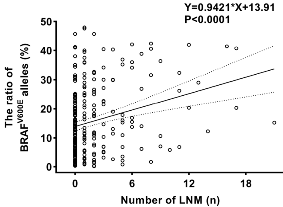
Figure 4. Correlation between BRAFV600E alleles ratio and the number of lymph node metastases in PTC. Note: Scatter plot shows the correlation of the ratio of BRAFV600E alleles and the number of LNM. Lines represent simple linear regression \pm 95\% confidence interval. Spearman's rho = 0.220, p < 0.0001 ; simple regression adjusted R^2 = 0.070 , p < 0.0001 .
