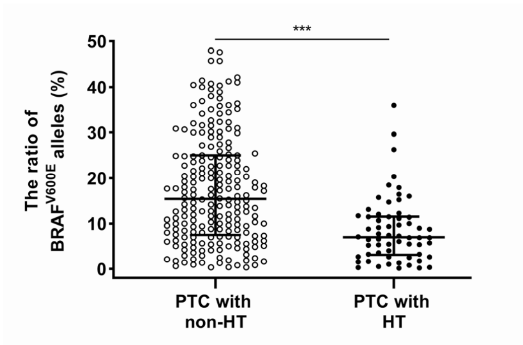
Figure 6. Comparison of BRAFV600E alleles ratio between Hashimoto's thyroiditis and those without in PTC. Note: ***: P value <0.001. Vertical scatter plots of the ratio of BRAFV600E alleles grouped by PTC combined Hashimoto's thyroiditis. Lines represent median and interquartile range.
