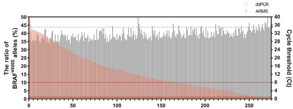
Figure 1. BRAFV600E mutation analysis in tissues sampled by ddPCR and ARMS in 275 PTC patients. The red bars indicate the ratio of BRAFV600E alleles detected by ddPCR (left Y-axis), in which 0.1% used as a cut-off value to define the BRAF-positive. The gray bars indicate the cycle threshold (Ct) detected by ARMS (right Y-axis). The red-thick line and fine line represent BRAFV600E alleles at ratio 1% and 10%, respectively. The gray dotted line indicates Ct value < 35 as a threshold to define the BRAF-positive by ARMS.
