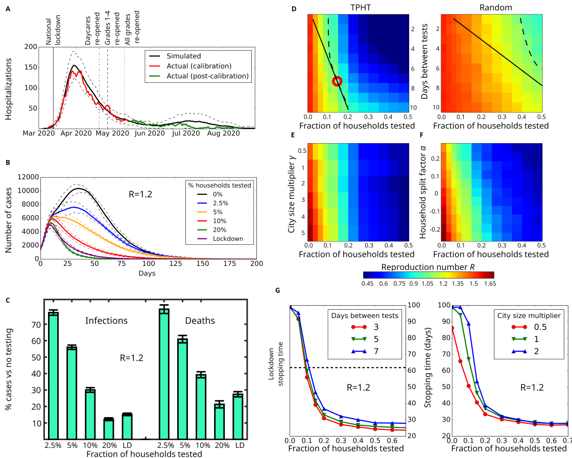
Fig. 2. Simulation results and effectiveness of targeted pooled household testing (TPHT) on COVID-19. (A) Fitting the model to Oslo hospitalization data. We plot the mean predicted number of hospitalizations (black) and confidence interval ( 2\sigma , dashed). Actual Oslo hospitalizations (red) were used as calibration (until May 15th). Hospitalization data May 15th- August 30th (green) were not used to determine model parameters. (B) Effect of TPHT in response to a sudden rise in cases (reaching 1,000 symptomatic individuals), assuming general infectivity parameters similar to those of Oslo in late May 2020 but with 50% increased infectivity of random contacts giving R = 1.2 . (C) Predicted number of deaths and infections for different TPHT testing fractions corresponding to panel (B), relative to no testing. Panels (D)-(F) use same parameters as panel (B), except with a 165% increased infectivity of random contacts giving
