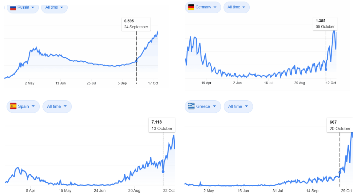
Figure 1: Typical examples of daily new COVID-19 cases (extracted from the Google home page when searching “covid”). All curves exhibit a clear boost of the growing rates.
