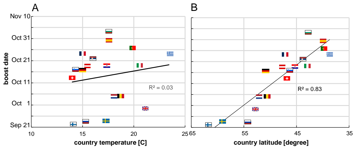
Figure 2: COVID-19 boost date as a function of the country mean temperature during the 2 preceding weeks (A), and as a function of the country PWC latitude (B) pointing vitamin D as one of the primary factor (flags link country between graphs).
