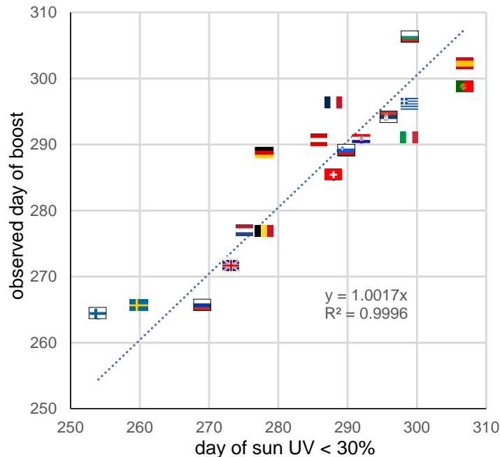
Figure 4: observed day of the second wave covid-19 boost as a function of the day when the country sun UV daily dose drops lower than 30% of that at latitude 0°. Trendline forced to intercept (0,0).
