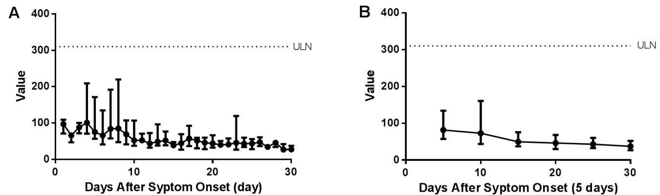
Fig. 1. The distribution over time of CK median in total cohort from symptom onset per day (A) and per 5 days (B).
