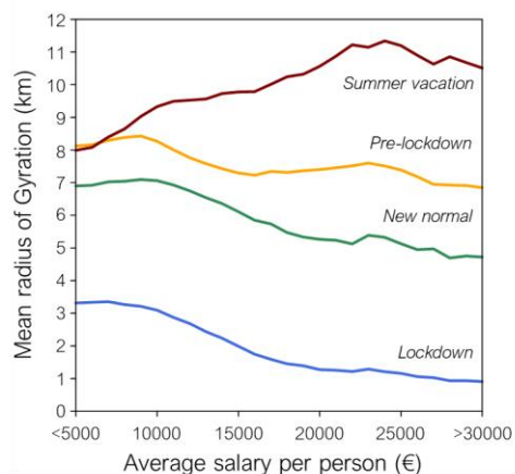
Fig. 3. Mean radius of gyration for the four periods defined by collective mobility patterns (see text for details).
