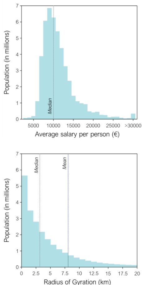
Fig. 1. Distribution of the average salary per person assigned by place of residence and distribution of the radius of gyration for all Spanish population.
