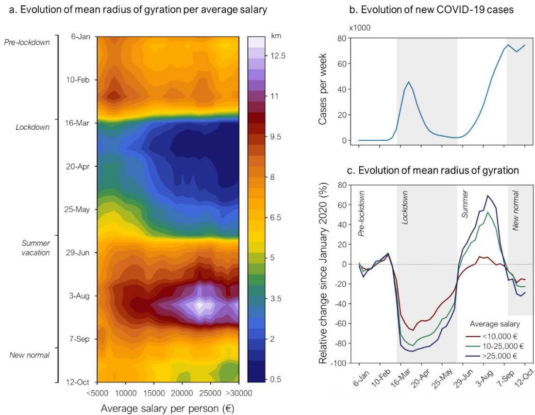
Fig 2. a. Evolution of mean radius of gyration per average salary for every week of 2020 until week 42 (starting at Monday 12th October). We can differentiate four clear periods according to mobility patterns: pre-lockdown, lockdown, summer holidays and new normal (see text for details). b. Evolution of the number of new COVID-19 cases for the same period. Remarkably, the same four periods are fitted by the curve. c. Evolution of the mean radius of gyration per average salary aggregated. It refers to i) 50% of the population with lower salary (<10,000€), ii) the top highest salaries (>25,000€) and, iii) the rest (10-25,000€).
