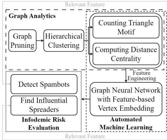
Fig. 1. An overview depicting the interdependence among the tasks solved by the MEGA framework for infodemic risk management.
