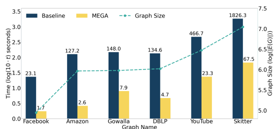
Fig. 17. Comparison between MEGA and the algorithm in [44] (which we set as baseline) on six social networks. The primary y-axis (blue) is the running time t in seconds, and the secondary y-axis (green) is the graph size |E(G)| . A log scale is used for these two axes, and we multiply t by 10 to avoid negative values (i.e., primary = \log(10 \cdot t) seconds and secondary = \log(|E(G)|) ). The number on top of each bar is the exact running time of both algorithms.
