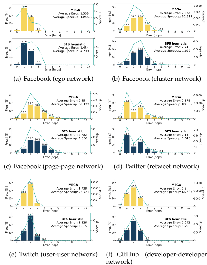
Fig. 20. Histograms of the error for MEGA (yellow) and the BFS heuristic in [7] (blue) on six different types of social networks with 100 vertices received the message in the spread graph. The green dotted line is the average speedup for each error and the average error is the average distance (in terms of hop count) between the real source and the estimators calculated by both methods over 500 simulations.
