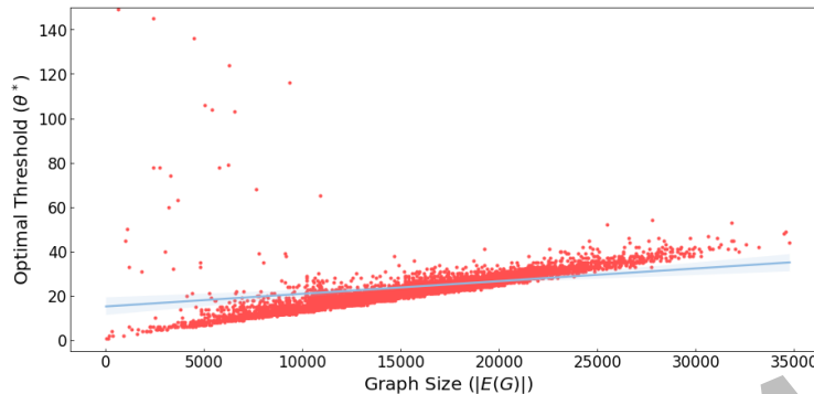
Figure 8: Optimal threshold tuning on 6,000 synthetic networks based on Lemma 1. The y-axis is the value of the optimal threshold \theta^* , and the x-axis is the graph size |E(G)| of each network. The blue line is a linear regression model that fits the results.
