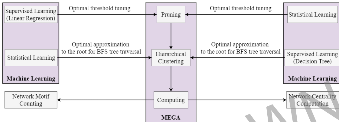
Figure 1: Overview of MEGA applied to solve the network motif counting (left) and network centrality computation (right). We use machine learning approaches to perform parameters tuning so as to optimize the performance of MEGA. The threshold \theta in the pruning step and the root in the hierarchical clustering step are two critical parameters that can significantly affect the overall performance of MEGA. For network motif counting, we use linear regression to compute an optimal threshold \theta^* and find an optimal approximation to the root based on the statistical features underlying graph data. We then use statistical data analysis to obtain \theta^* for network centrality computation and apply decision tree algorithm to find an optimal root for MEGA.
