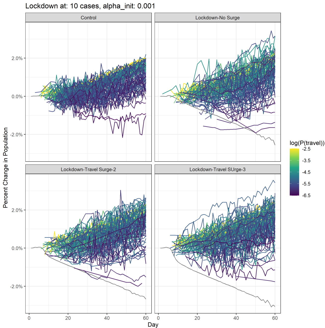
Figure S1. Depopulation of urban center with \alpha_0 of 0.001.
