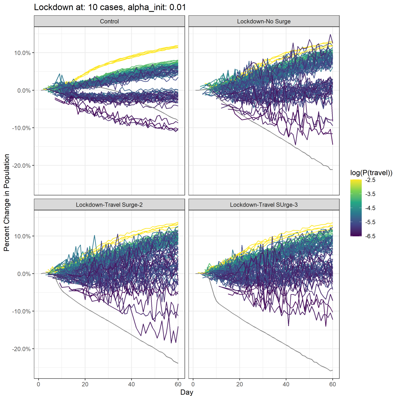
Figure S3. Depopulation of urban center with \alpha_0 of 0.01.
