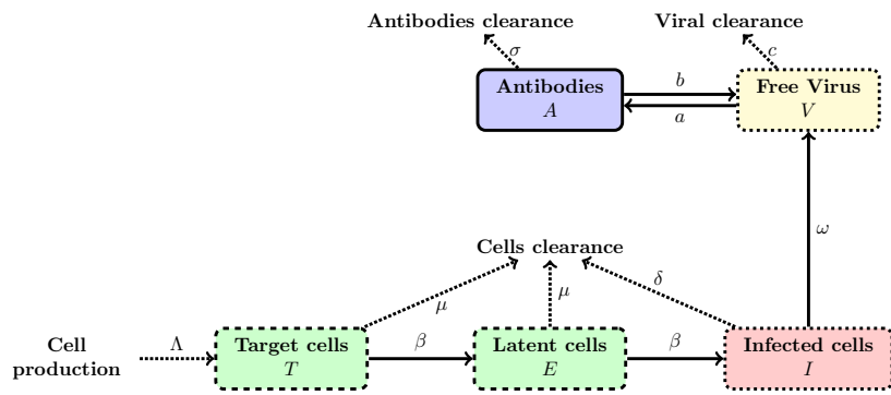
Figure 8: Graphical illustration of the flow in the model (29)-(34).
