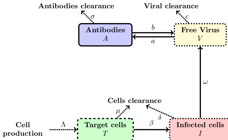
Figure 1: Graphical illustration of the flow in the model (1)-(5).
