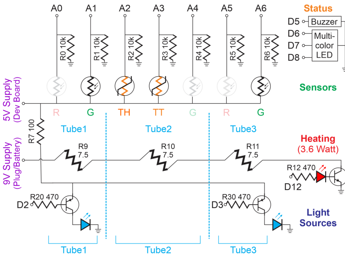
Figure 1. The circuit diagram. A0-A6 are the analog inputs and D2, D3, D5-D8, D12 are digital pins outputs of the Arduino nano. Note the transistor near R12 is an NPN BJT while the two transistors near R20 and R30 are PNP BJTs. The diagram shown allows for the system to be easily converted into a two-color fluorescence system (those elements are grayed out and are not necessary for the primary build in this paper). Each tube position is also indicated showing which components relate to which reaction tube.
