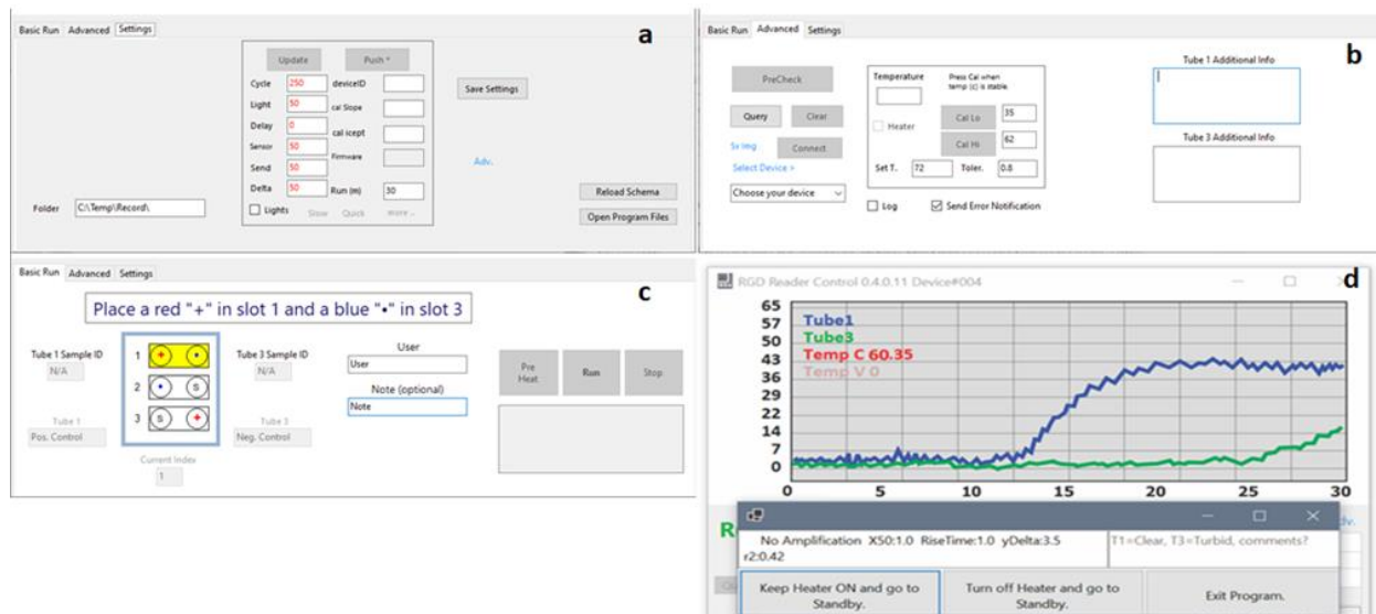
Figure 7 Software. A. Settings tab of the reader software. This tab contains the device ID information as well as calibration settings and pin designations. The destination of the run data is designated here. B. Advanced tab of the software. The advanced tab contains thermistor calibration inputs as well as device selection and metadata input. C. “Basic run” tab of the software. Following quality control all testing will be facilitated here through following the software guided instructions. Additional information such as the sample ID, user, and notes can
