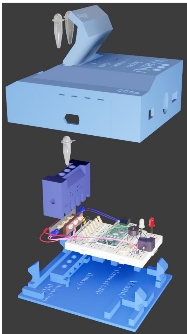
Figure 5. View of all components. From the bottom up, you can visualize the pieces and how they fit together. Bottom is the “base” 3-D printed part, then the electronics boards. Then the tube holder, then tube thermistor, then the “enclosure”, then the reaction tubes, then the lid. This ordering is not precise to the build, since the tube holder is assembled before all the connections to the electronics. The middle tube is separated from the outer tubes since this tube is used for the temperature control (in-tube thermistor) and is placed and tested before the top enclosure is fitted.
