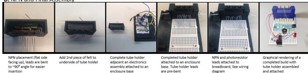
Figure 4 Instructions for Tube Holder construction. A Photoresistors, thermistor, and emission filter insertion. B Heating element construction. C Heating element insertion to the holder. D NPN and final assembly.
