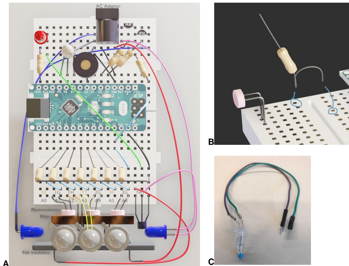
Figure 2. Graphical rendering of the electronics. A. An overhead view of the electronics. The controller (Arduino Nano) is centrally located spanning the two 170 tie breadboards. The top of the image depicts the back of the reader assembly. This area houses the status indicators such as the status LED (white with leads to D6, D7, D8) and buzzer (black ring to D5). This section also contains the heating indicator (red LED), light controls (PNPs), and AC adaptor. A 470-ohm resistor connects digital pin D12 to the red LED, which is then jumped down to the base of the NPN. The lighting control components are PNP transistors whose base is connected to digital pins D2 and D3 by 470-ohm resistors on the upper right along with their collectors to jumper wires connecting to the LED lights. A 100-ohm resistor paired with a jumper wire provides 5-volt power from the controller to the PNPs' common emitters. The bottom of the image displays the front of the electronics featuring the sensor array that attaches to the tube holder (assembly shown in Figure 4 ). Sensors are powered by the controller's 5-volt supply, which vary their resistance for either light or temperature, then go to analog pins A0 through A6 and have a parallel path through a 10K-ohm resistor to ground. The ground and 5-volt rails are extended to the outer board via the jumper wires shown. NPN transistor is also depicted with its leads: Collector, Base, Emitter from left to right. B. Single resistor bridge depiction. Folding of the resistor lead enables it to be used as a bridge to connect the sensor rail to the proper analog pin of the controller. Forceps or fine nose pliers can be used to create the fold. C. In-Tube thermistor.
