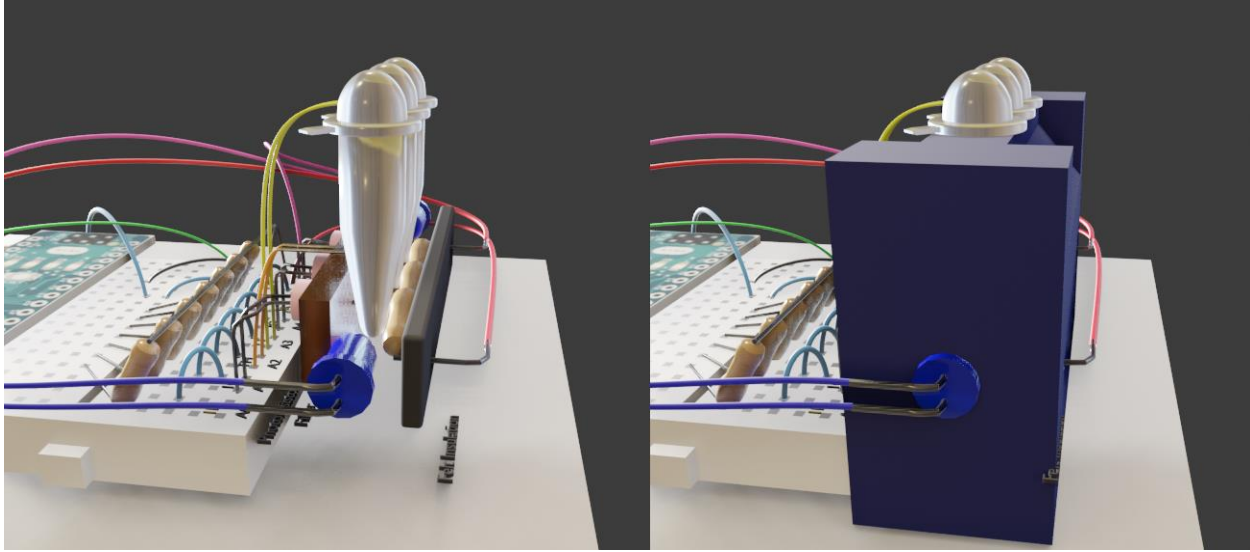
Figure 3. A side view of the components inside the “tube holder”. Contained within the tube holder is the heating element, in-holder thermistor, in tube thermistor, blue LEDs, and photoresistors. Clips are present to hold both the filter and heating element insulation in place. Additionally, a blue emission filter is placed in front of the photoresistors.
