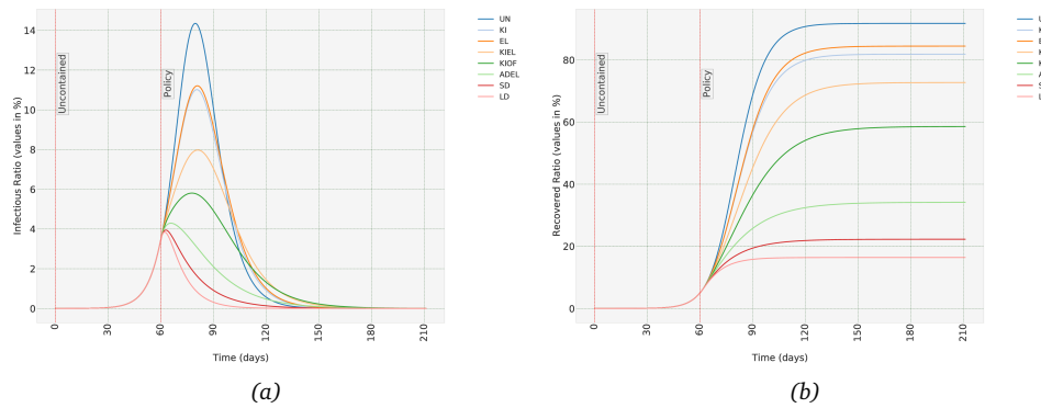
Figure 2: Effects of different suppression policies (as defined in Table 2) in Germany, when population is uncontained for the first 60 days of the spread of the virus. (a) Infectious (b) Recovered trajectory.
