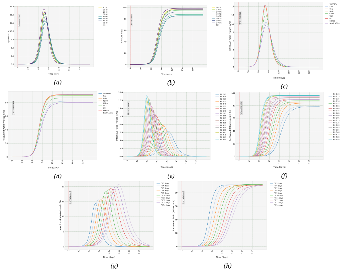
Figure 1: Uncontained scenario: (a,b) The Infectious and Recovered trajectories in the uncontained population in each age-group in Germany, (c,d) Aggregate trajectories of Infectious and Recovered in different countries. (e,f) Aggregate trajectories of Infectious and Recovered in Germany when R_0 in uncontained population assumes different values, (g,h) Aggregate trajectories of Infectious and Recovered in Germany with different values of T_i (the average time-period hosts remain infectious).
