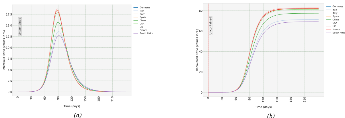
Figure 5: (a) The uncontained scenario in different countries assuming SARS-CoV-2 dynamics follow an SIR model, not an SEIR model, (a) Aggregate ratio of Infectious compartment, (b) Aggregate ratio of Recovered compartment.
