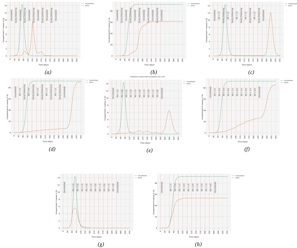
Figure 3: The effects of long-term strategies on Infectious and Recovered trajectories when we switch between policies of different degrees of severity. Policies as defined in Table 2: (a,b) Switching between uncontained and social-distancing scenarios, (c,d) A less strict long-term strategy when we switch between social distancing and R_0 = 1.5 scenarios, (e,f) switch between situations where R_0 = 0.9 and R_0 = 1.5 . Containment policy can contain the spread of the virus when imposed 30 days after 1 in 100,000 in population is Infectious, (g,h) Same as in Figure 3e, only difference is that policy is imposed 60 days after Infectious population reaches 1 in 100,000. An extra 30 days of inaction causes the ratio of Infectious to reach a peak of 5.58%.
