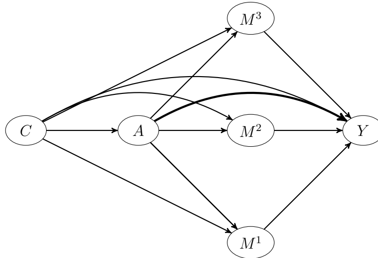
Figure 1: DAG showing causal structure linking exposure, mediators and outcome
