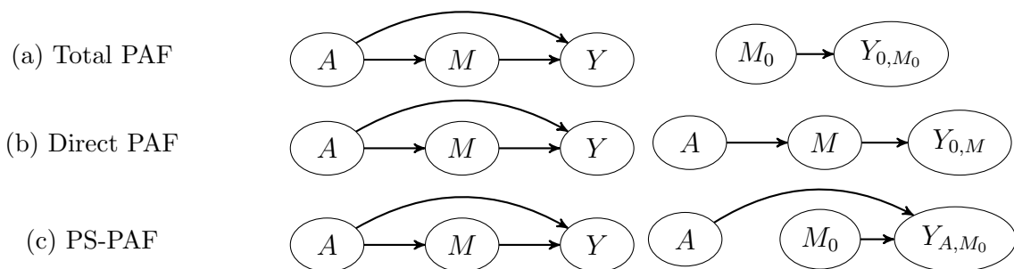
Figure 2: Illustration of total, direct and pathway specific PAF as a comparison between disease risk in current population (graph on LHS) and counterfactual disease risk in a population where particular pathways through which the risk factor effects disease are disabled (graph on RHS). A situation with a single mediated pathway A \rightarrow M \rightarrow Y is illustrated. Sub-figure (a) Total PAF compares observed disease risk P(Y = 1) vs disease risk P(Y_{0,M_0} = 1) in a hypothetical population where both direct and mediated pathways are disabled. Sub-figure (b) Direct PAF compares observed disease risk vs disease risk P(Y_{0,M} = 1) in a hypothetical population where the direct pathway is disabled. Sub-figure (c) Pathway specific PAF compares observed disease risk Y vs disease risk P(Y_{A,M_0} = 1) in a hypothetical population where the mediated pathway A \rightarrow M \rightarrow Y is disabled
