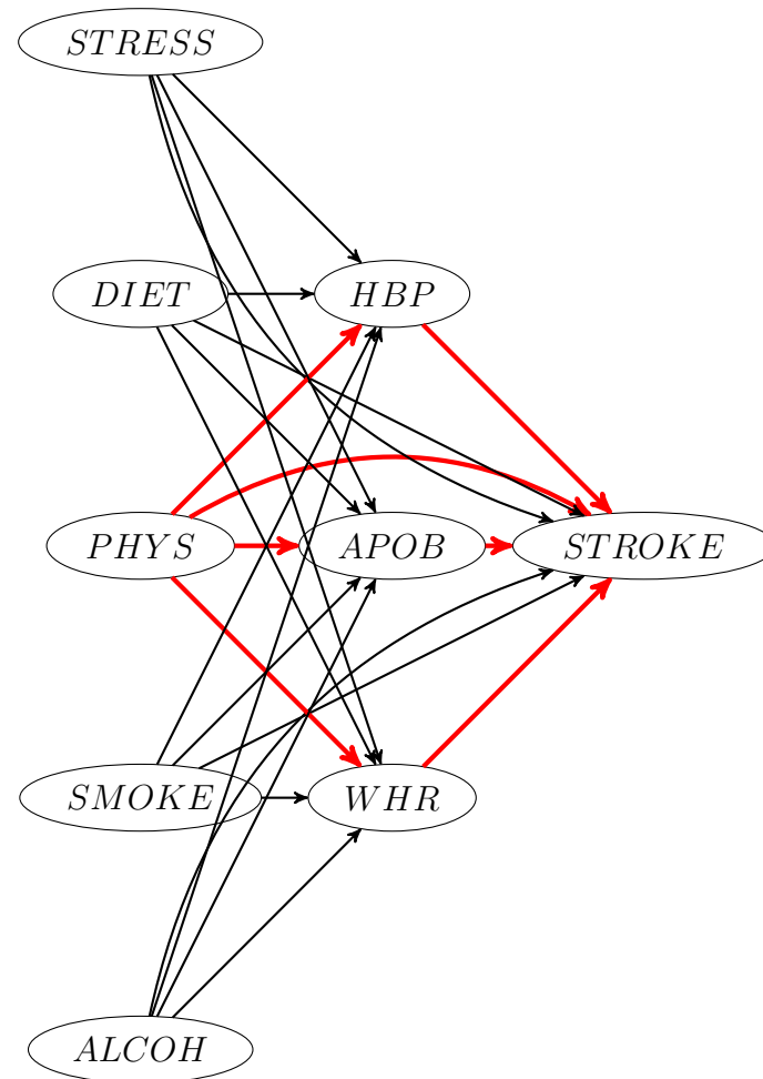
Figure 4: DAG showing assumed causal structure for risk factors in INTERSTROKE. The direct and mediating pathways associated with physical activity are highlighted in bold red. Age, sex and geographic region are confounders for the risk/factor disease relationship for all listed factors on the figure (these are omitted for display purposes)
