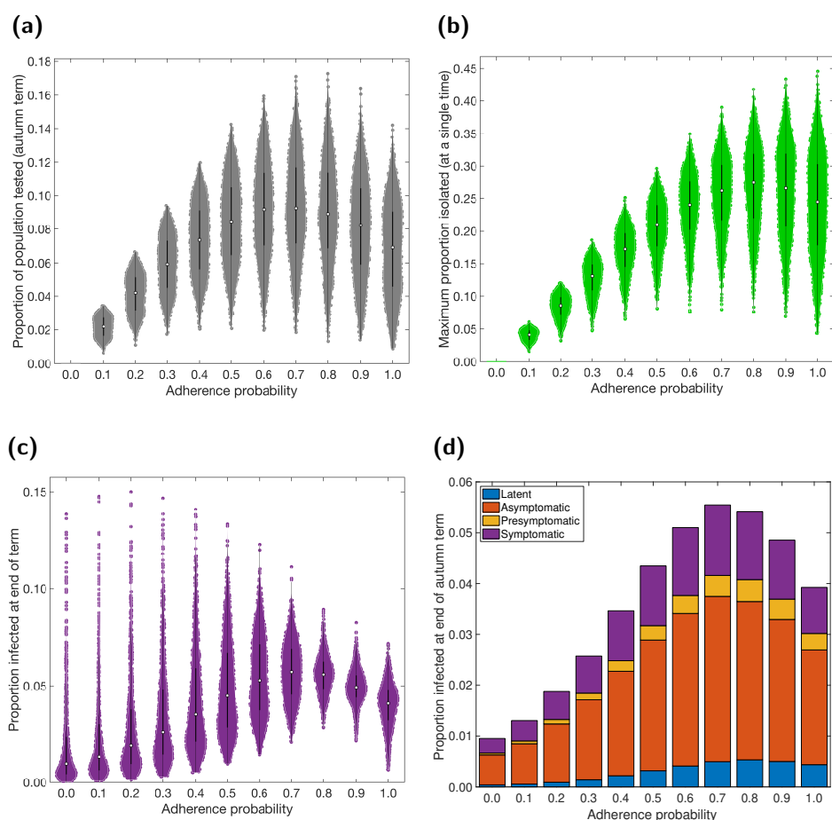
Fig. 5: Cumulative epidemiological measures over the autumn term under differing levels of adherence to nonpharmaceutical interventions. Outputs summarised from 1,000 simulations (on 50 network realisations with 20 runs per network) for various levels of adherence to nonpharmaceutical interventions. White markers denote medians and solid black lines span the 25th to 75th percentiles. (a) Proportion of population infected by SARS-CoV-2 and tested. (b) Maximum proportion of students isolated at any single time. (c) Proportion of students infected at the end of the autumn term. (d) Under each level of adherence, median proportion of student population in latent (blue), asymptomatic (orange), presymptomatic (yellow), symptomatic (purple) infected states at the end of the autumn term. For percentile summary statistics, see Table S4.
