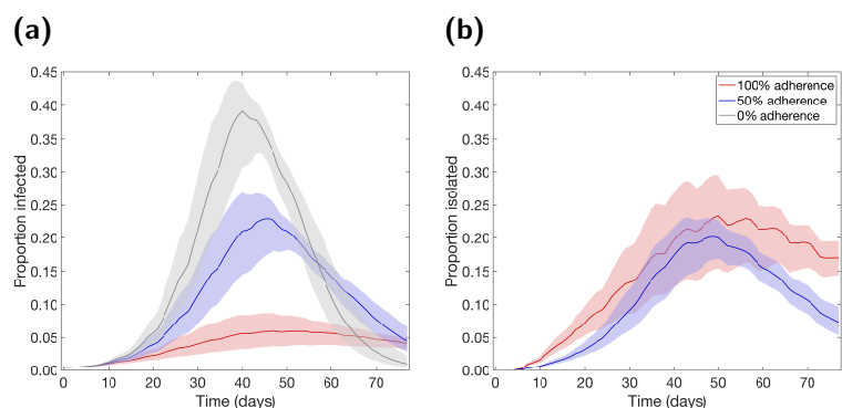
Fig. 4: Temporal profiles of epidemiological measures over the autumn term under differing levels of adherence to nonpharmaceutical interventions. Outputs produced from 1,000 simulations (with 20 runs per network, for 50 network realisations) for three levels of adherence to nonpharmaceutical interventions: 0% (grey), 50% (blue), 100% (red). Solid lines depict the median profile and shaded regions the 50% prediction interval. Patterns of infection prevalence and proportion of the student community in isolation demonstrated trade-offs between case numbers and the need for portions of the population to isolate. (a) Proportion infected. (b) Proportion isolated.
