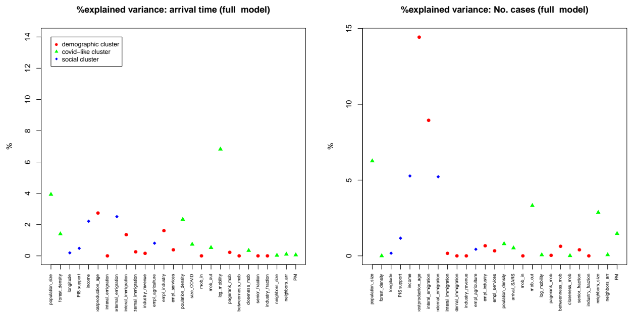
Figure 2. Predictive model (Multiple linear regression) of arrival times (left - the model gives 29% explained variance) and number of cases (right - the model gives 53% explained variance) on all non-collinear (linear combinations of other variables) variables. The y-axis shows the % of explained variance for each of the variables from the x-axis. The points are marked and colored according to the PCA classification (as in the same single legend for both charts)
