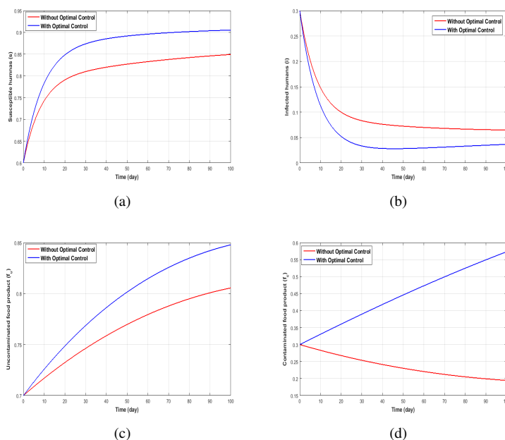
Figure 10 Dynamics with permissible controls u_2 = u_3 \neq 0 for (a) Susceptible (b) Infected (c) Untaminated food (d) Contaminated food
