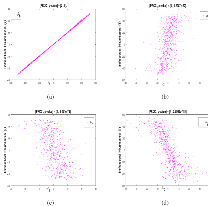
Figure 3 (a) and (b) Scatter plots of parameters loss of immunity rate ( \rho_h ) and human recovery rate \alpha with positive PRCC. (c) and (d) Scatter plots of parameters human infection rate of Listeriosis ( \omega_1 ) and rate of uncontaminated food contamination by L. Monocytogenes ( \omega_2 ) with negative PRCC.
