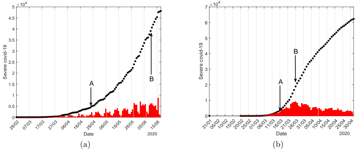
Figure 3: The daily (bars) and the accumulated (points) severe covid-19 cases in São Paulo State (a) and Spain (b), where A indicates the time at which quarantine was introduced, and B indicates the time at which the inflexion point occurred.
