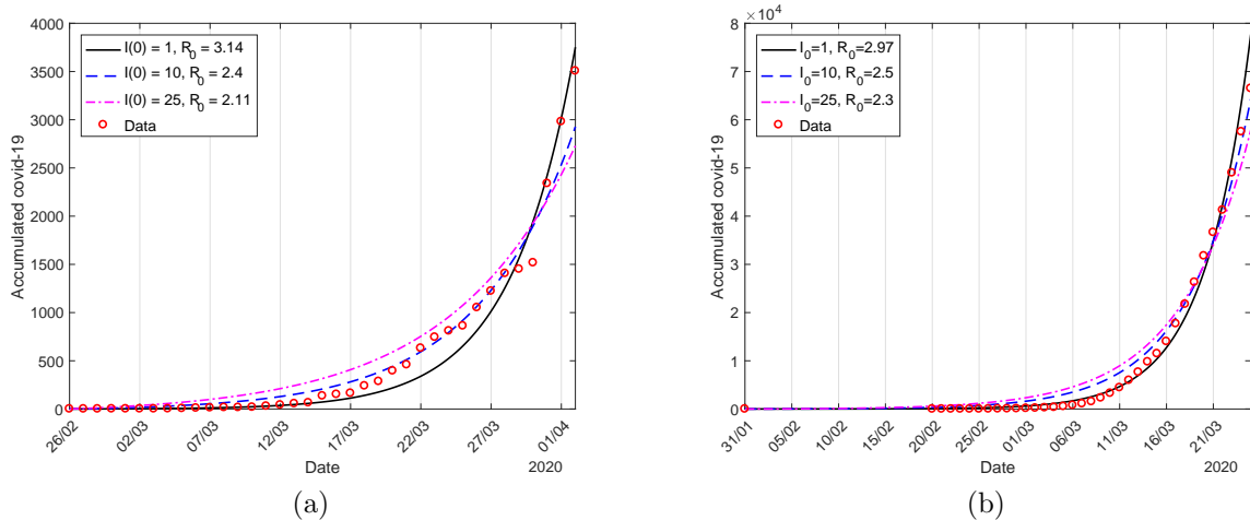
Figure 1: The estimated curve \Omega for São Paulo (a) and Spain (b) with three different initial conditions I(0) = 1 (continuous curve), 10 (dashed curve), and 25 (dashed and dotted curve).
