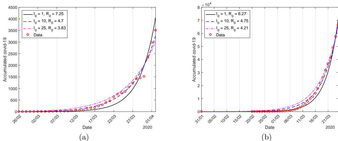
Figure C.1: The estimated curve \Omega for São Paulo (a) and Spain (b) with three different initial conditions I(0) = 1 (continuous curve), 10 (dashed curve), and 25 (dashed and dotted curve).
