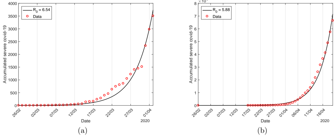
Figure 2: The estimated curve \Omega and the observed accumulated cases for São Paulo State (a) and Spain (b).
