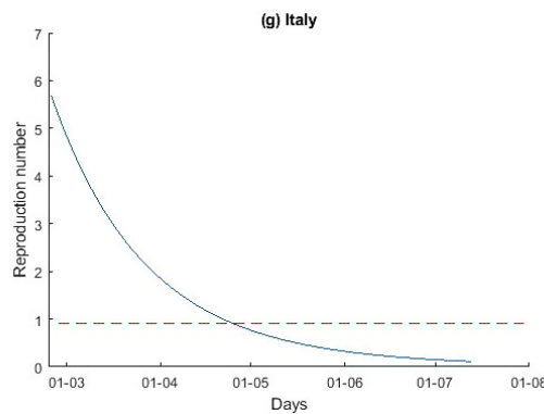
Figure 2 Estimated effective reproduction number over time
