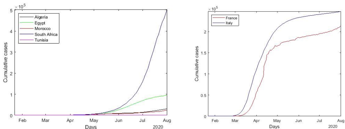
Figure 1 Cumulative reported cases of COVID-19 disease.
