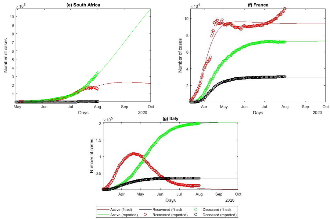
Figure 3 COVID-19 epidemiological data reported and fitted by SEIRQDP model
