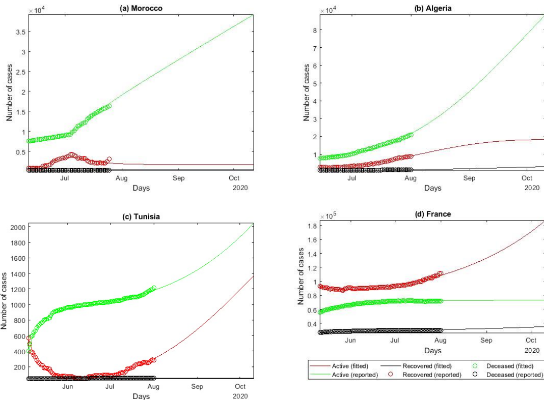
274 Figure 4 COVID-19 epidemiologic data reported and fitted by SEIQRDP model after the lockdown lifting.
