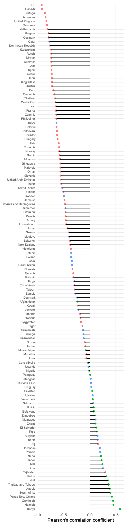
Fig. 3 Pearson's correlation coefficient of the association between the effective reproduction number and the stringency index by country Note. Positive correlation values suggest that a high stringency was favoring disease spread.
