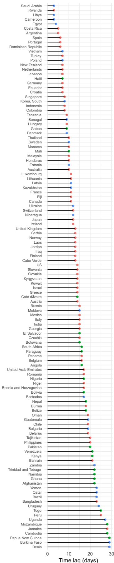
Fig. 2 Estimated time lag by country Note. The following countries had a p-value > 0.05 of the regression model of their effective reproduction number on lagged mobility, and were so excluded: Sri Lanka, Mongolia, Mauritius, Taiwan, and Zimbabwe.
