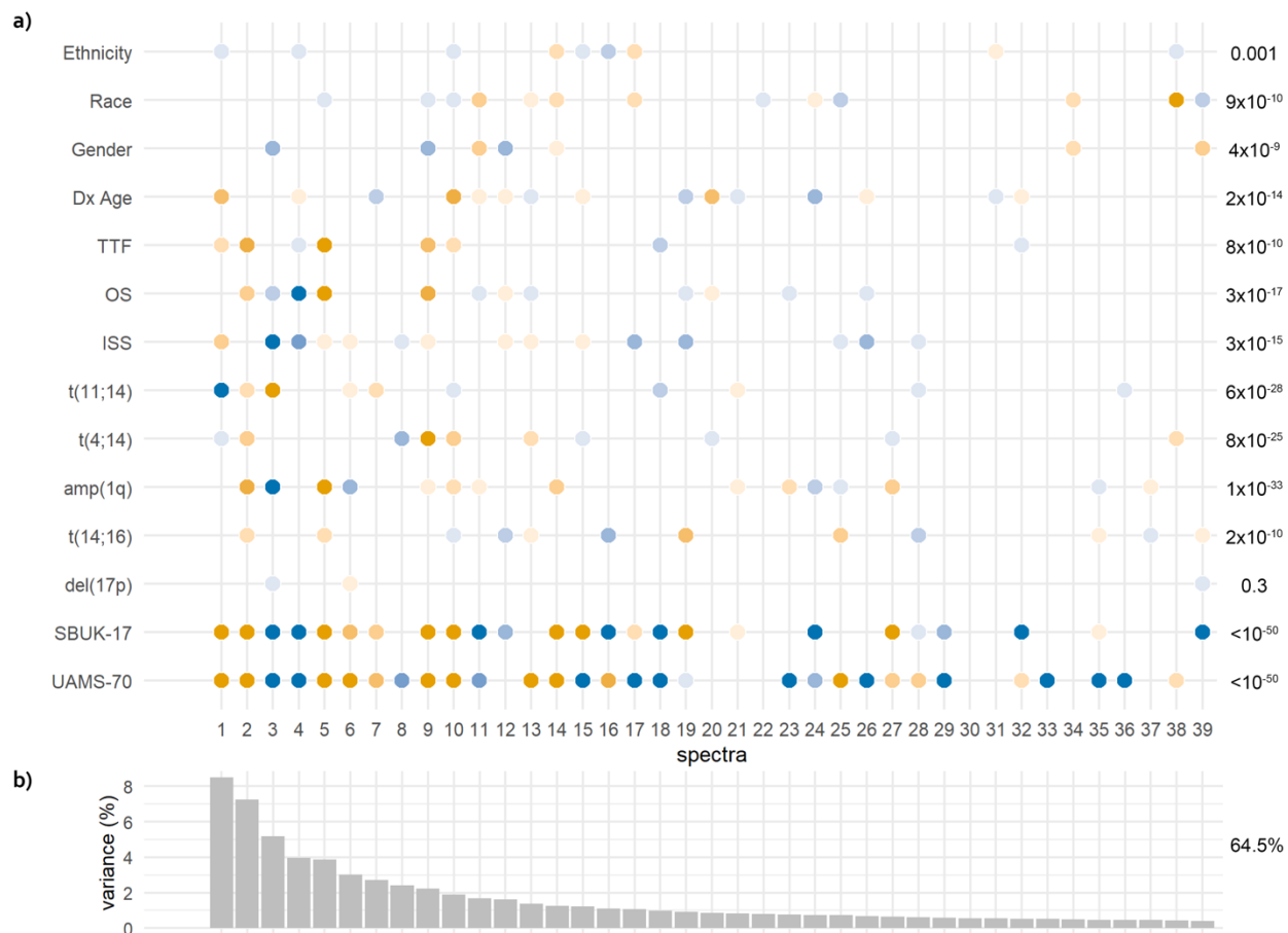
Figure 4. Overview of CD138+ spectra outcome modeling. a) Multivariable modeling results. The outcome of interest (left y-axis) and the significance of the full 39-spectra model (right y-axis). Spectra variables are illustrated on the x-axis. The significance and direction of each spectrum are indicated: blue negative beta coefficient, orange positive beta coefficient. No dot is shown if a spectrum was not significantly associated at p < 0.05 level. b) Percent of the global variance captured by each spectra variable. The total variance captured by all 39 spectra is shown at the right.
